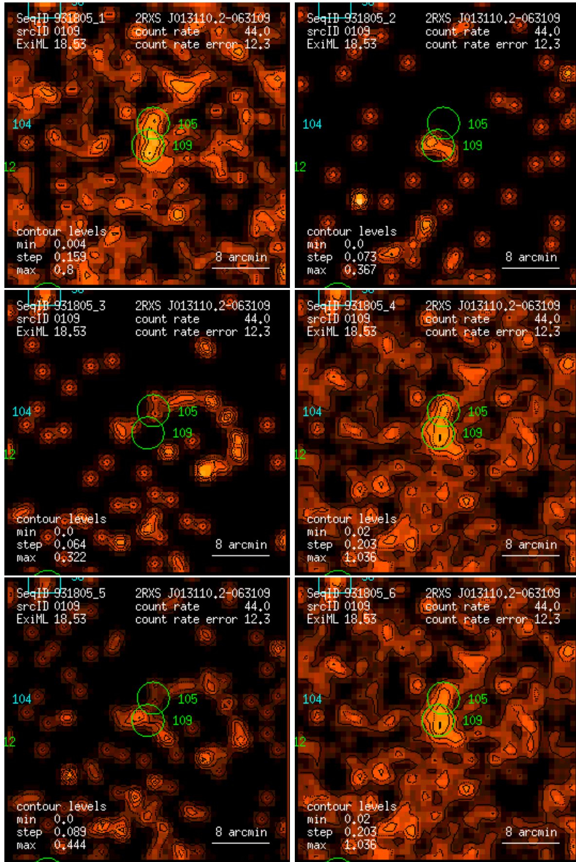
Figure 109: RASS 931805: detection 0109: band rate images, Gaussian filter: (1) PSPC channels 11 – 41, (2) 52 – 90, (3) 91 – 201, (4) 11 – 235, (5) 52 – 201, (6) 11 – 201. Broad band rates in counts/ks. Band rate contour levels in counts/ks/arcmin 2 .
