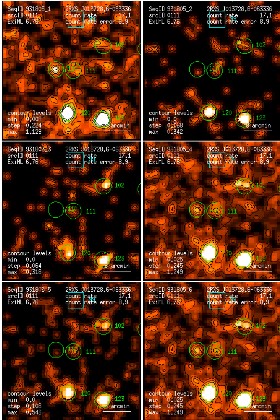
Figure 111: RASS 931805: detection 0111: band rate images, Gaussian filter: (1) PSPC channels 11 – 41, (2) 52 – 90, (3) 91 – 201, (4) 11 – 235, (5) 52 – 201, (6) 11 – 201. Broad band rates in counts/ks. Band rate contour levels in counts/ks/arcmin 2 .
