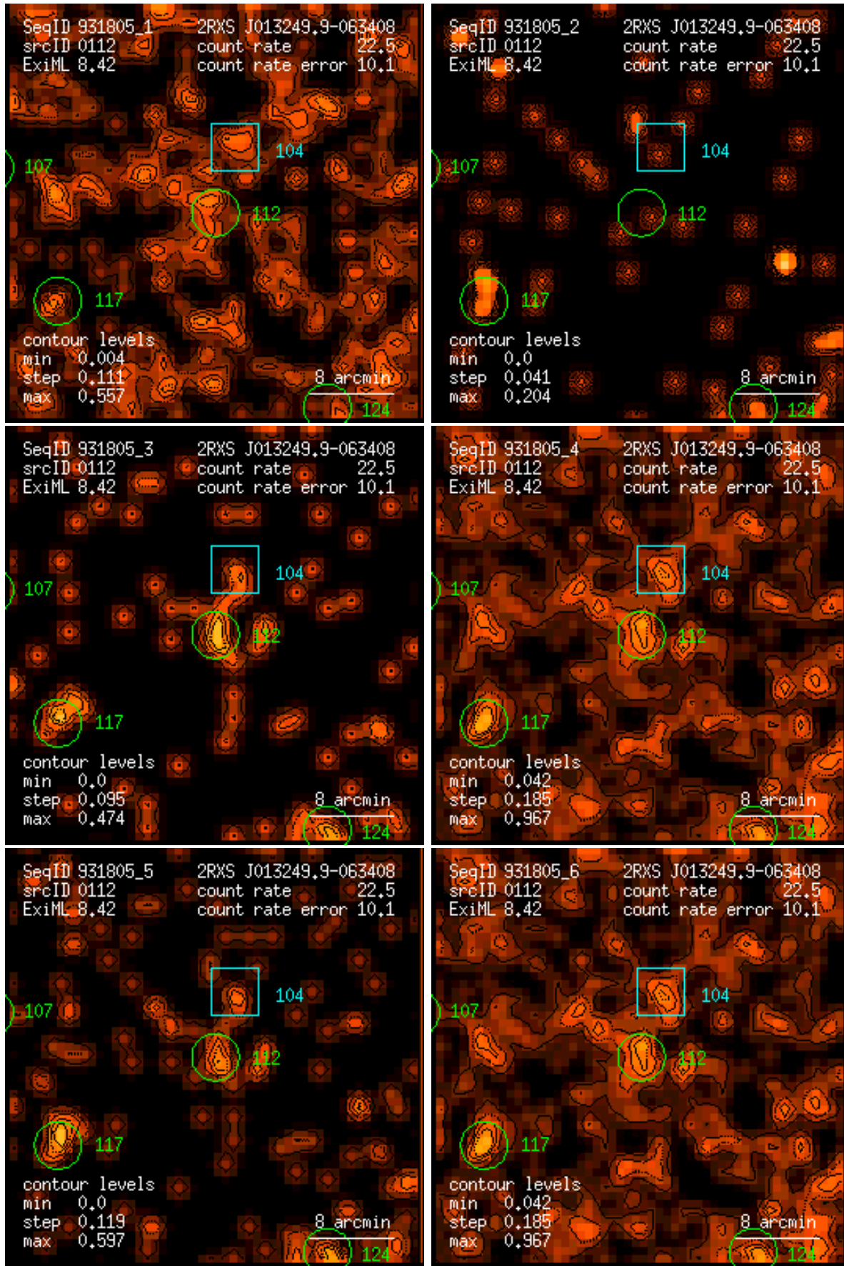
Figure 112: RASS 931805: detection 0112: band rate images, Gaussian filter: (1) PSPC channels 11 – 41, (2) 52 – 90, (3) 91 – 201, (4) 11 – 235, (5) 52 – 201, (6) 11 – 201. Broad band rates in counts/ks. Band rate contour levels in counts/ks/arcmin 2 .
