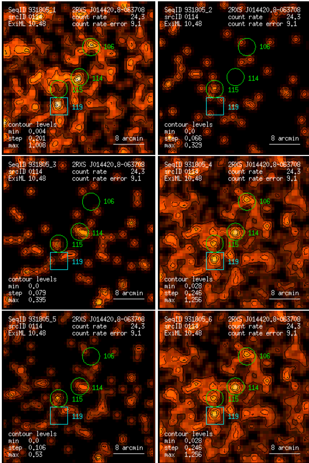
Figure 114: RASS 931805: detection 0114: band rate images, Gaussian filter: (1) PSPC channels 11 – 41, (2) 52 – 90, (3) 91 – 201, (4) 11 – 235, (5) 52 – 201, (6) 11 – 201. Broad band rates in counts/ks. Band rate contour levels in counts/ks/arcmin 2 .
