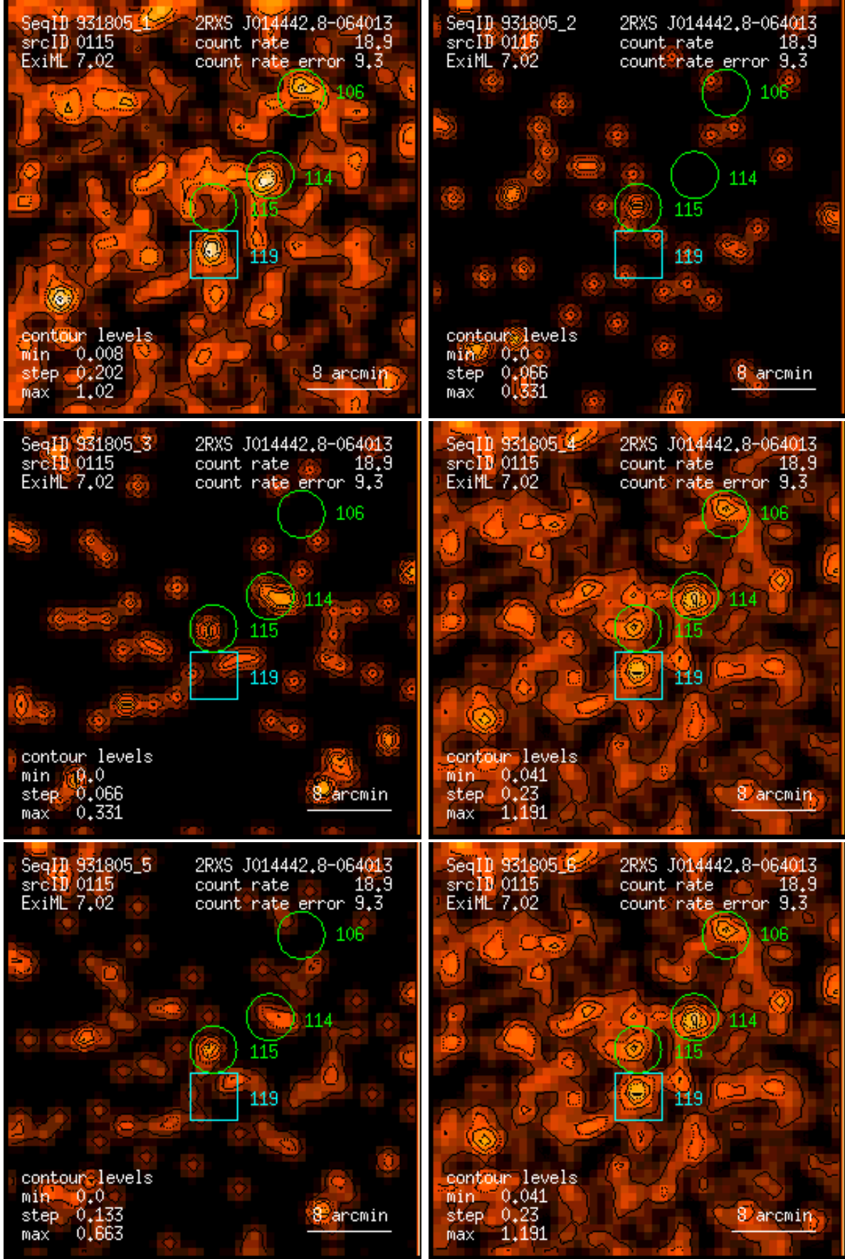
Figure 115: RASS 931805: detection 0115: band rate images, Gaussian filter: (1) PSPC channels 11 – 41, (2) 52 – 90, (3) 91 – 201, (4) 11 – 235, (5) 52 – 201, (6) 11 – 201. Broad band rates in counts/ks. Band rate contour levels in counts/ks/arcmin 2 .
