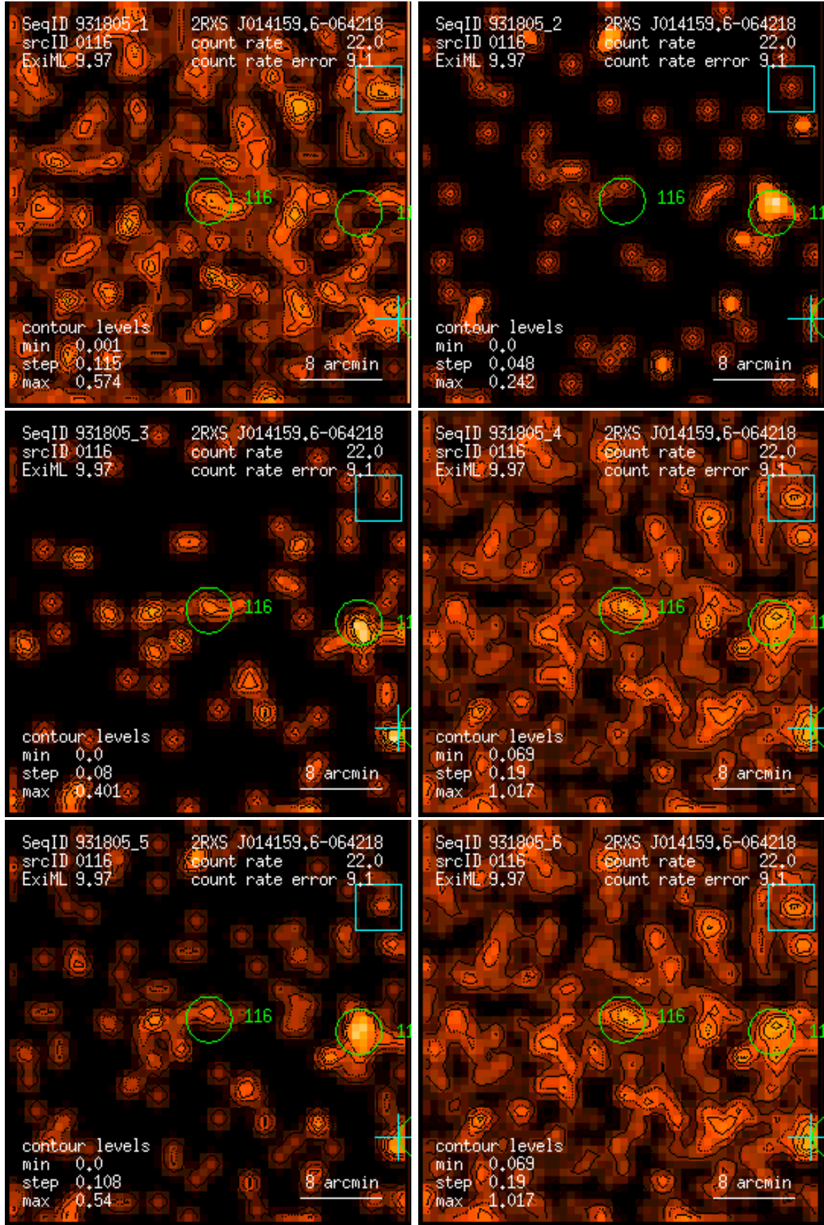
Figure 116: RASS 931805: detection 0116: band rate images, Gaussian filter: (1) PSPC channels 11 – 41, (2) 52 – 90, (3) 91 – 201, (4) 11 – 235, (5) 52 – 201, (6) 11 – 201. Broad band rates in counts/ks. Band rate contour levels in counts/ks/arcmin 2 .
