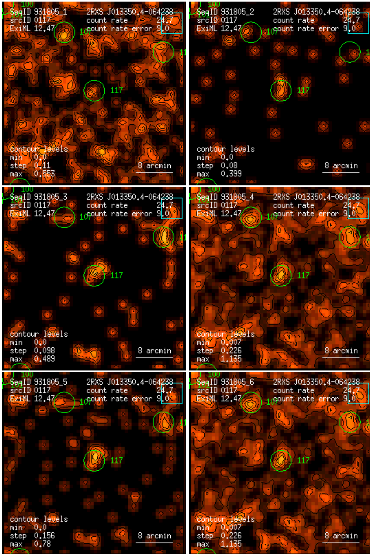
Figure 117: RASS 931805: detection 0117: band rate images, Gaussian filter: (1) PSPC channels 11 – 41, (2) 52 – 90, (3) 91 – 201, (4) 11 – 235, (5) 52 – 201, (6) 11 – 201. Broad band rates in counts/ks. Band rate contour levels in counts/ks/arcmin 2 .
