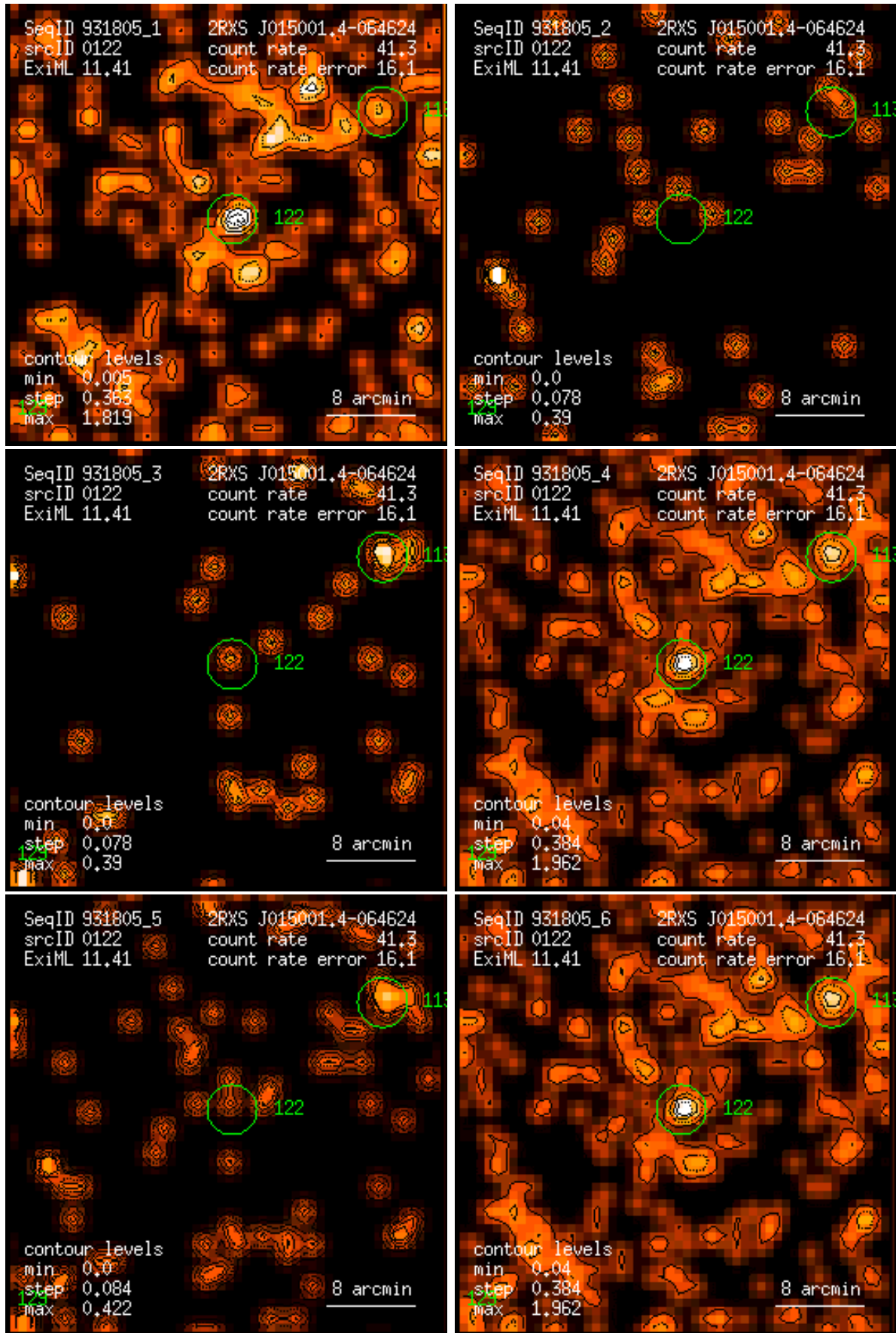
Figure 122: RASS 931805: detection 0122: band rate images, Gaussian filter: (1) PSPC channels 11 – 41, (2) 52 – 90, (3) 91 – 201, (4) 11 – 235, (5) 52 – 201, (6) 11 – 201. Broad band rates in counts/ks. Band rate contour levels in counts/ks/arcmin 2 .
