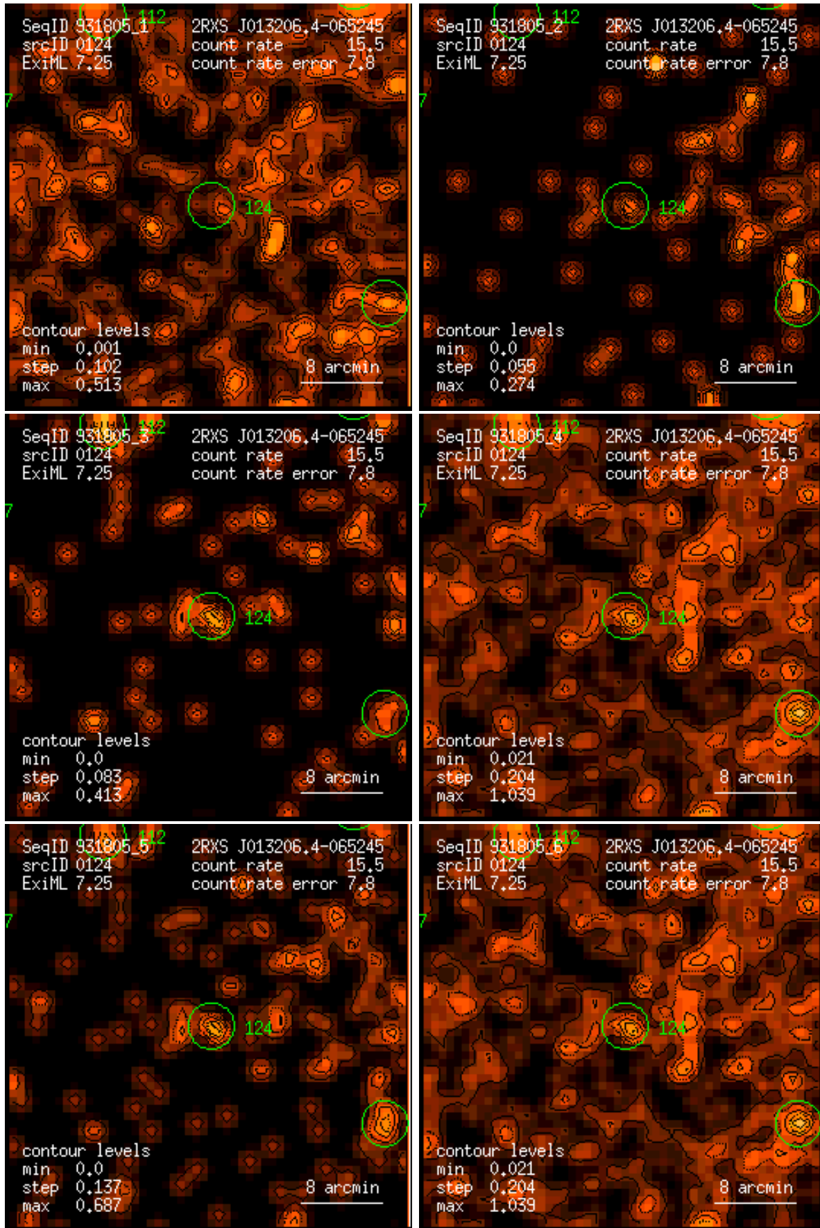
Figure 124: RASS 931805: detection 0124: band rate images, Gaussian filter: (1) PSPC channels 11 – 41, (2) 52 – 90, (3) 91 – 201, (4) 11 – 235, (5) 52 – 201, (6) 11 – 201. Broad band rates in counts/ks. Band rate contour levels in counts/ks/arcmin 2 .
