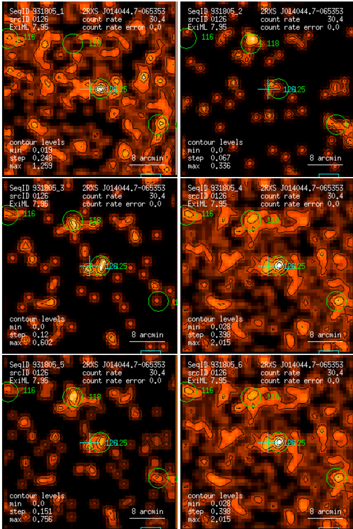
Figure 126: RASS 931805: detection 0126: band rate images, Gaussian filter: (1) PSPC channels 11 – 41, (2) 52 – 90, (3) 91 – 201, (4) 11 – 235, (5) 52 – 201, (6) 11 – 201. Broad band rates in counts/ks. Band rate contour levels in counts/ks/arcmin 2 .
