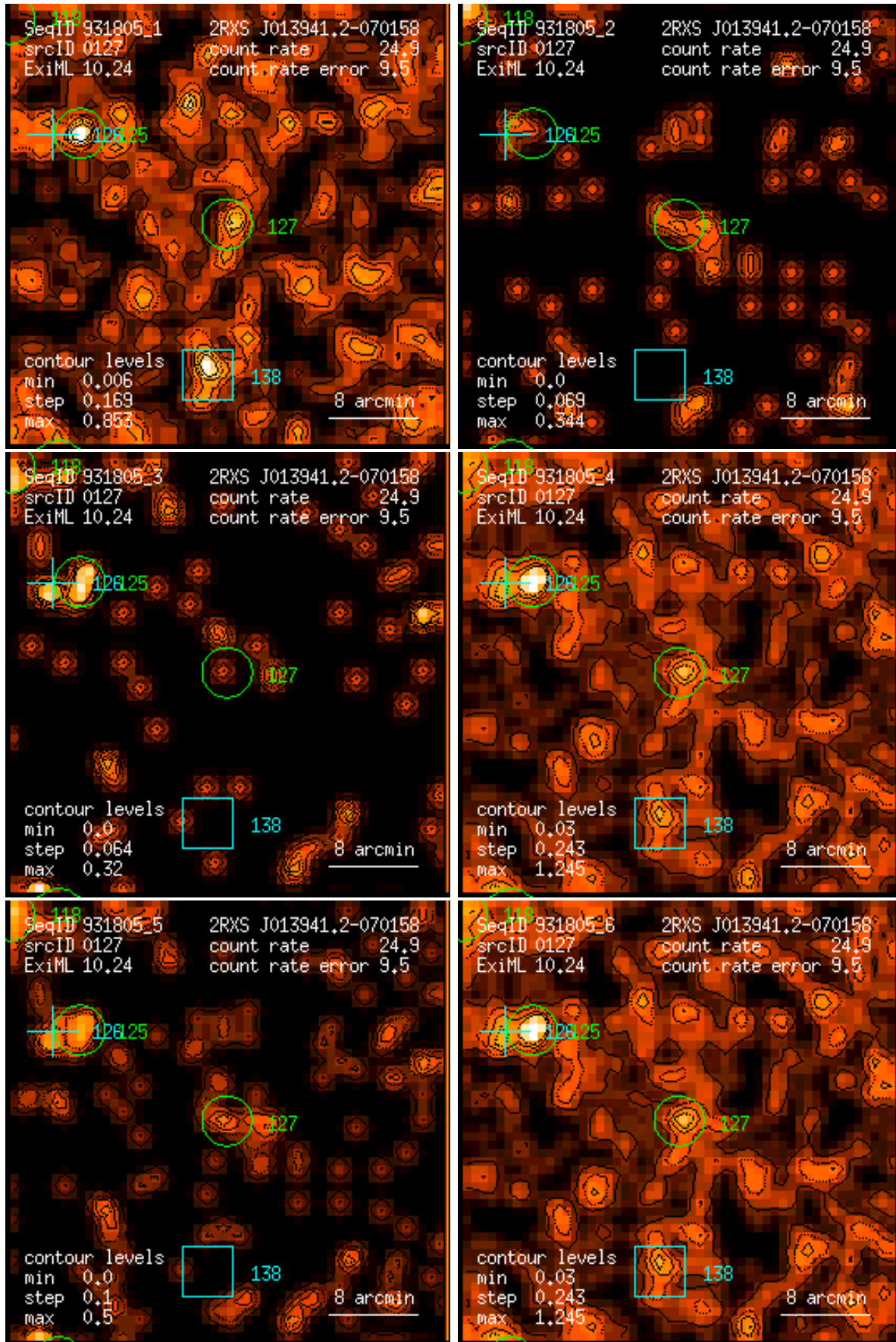
Figure 127: RASS 931805: detection 0127: band rate images, Gaussian filter: (1) PSPC channels 11 – 41, (2) 52 – 90, (3) 91 – 201, (4) 11 – 235, (5) 52 – 201, (6) 11 – 201. Broad band rates in counts/ks. Band rate contour levels in counts/ks/arcmin 2 .
