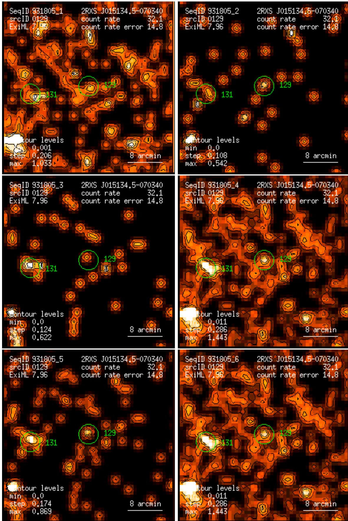
Figure 129: RASS 931805: detection 0129: band rate images, Gaussian filter: (1) PSPC channels 11 – 41, (2) 52 – 90, (3) 91 – 201, (4) 11 – 235, (5) 52 – 201, (6) 11 – 201. Broad band rates in counts/ks. Band rate contour levels in counts/ks/arcmin 2 .
