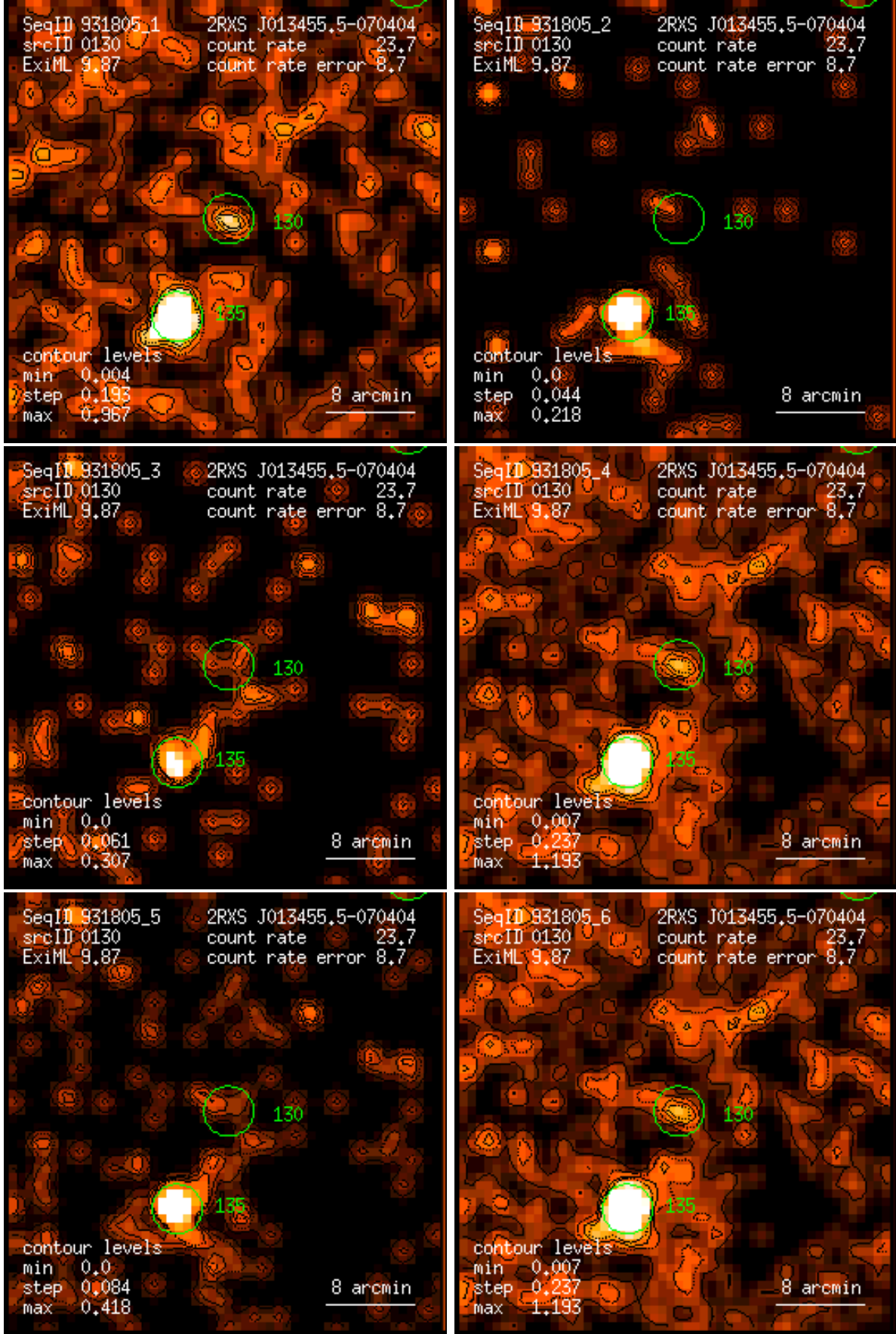
Figure 130: RASS 931805: detection 0130: band rate images, Gaussian filter: (1) PSPC channels 11 – 41, (2) 52 – 90, (3) 91 – 201, (4) 11 – 235, (5) 52 – 201, (6) 11 – 201. Broad band rates in counts/ks. Band rate contour levels in counts/ks/arcmin 2 .
