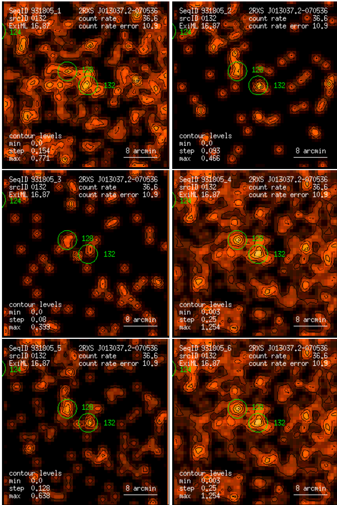
Figure 132: RASS 931805: detection 0132: band rate images, Gaussian filter: (1) PSPC channels 11 – 41, (2) 52 – 90, (3) 91 – 201, (4) 11 – 235, (5) 52 – 201, (6) 11 – 201. Broad band rates in counts/ks. Band rate contour levels in counts/ks/arcmin 2 .
