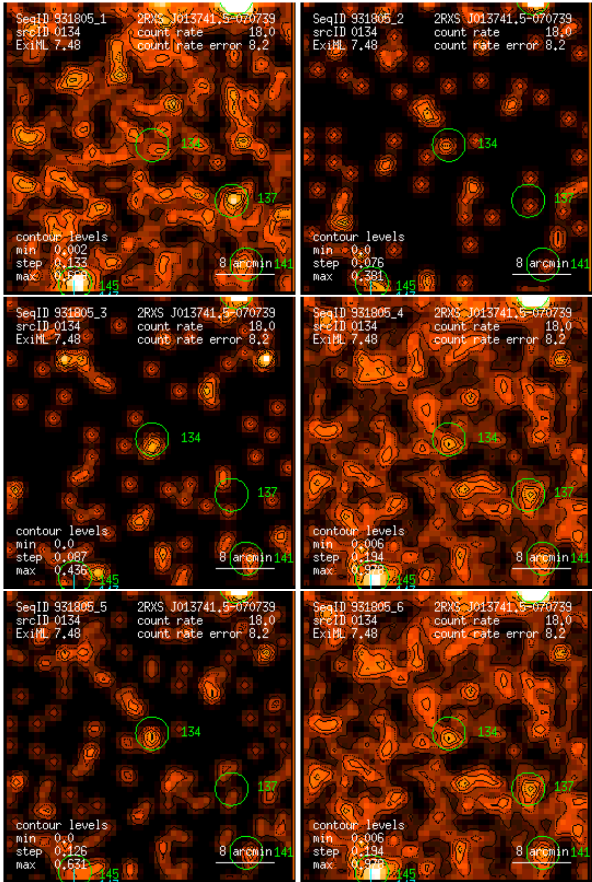
Figure 134: RASS 931805: detection 0134: band rate images, Gaussian filter: (1) PSPC channels 11 – 41, (2) 52 – 90, (3) 91 – 201, (4) 11 – 235, (5) 52 – 201, (6) 11 – 201. Broad band rates in counts/ks. Band rate contour levels in counts/ks/arcmin 2 .
