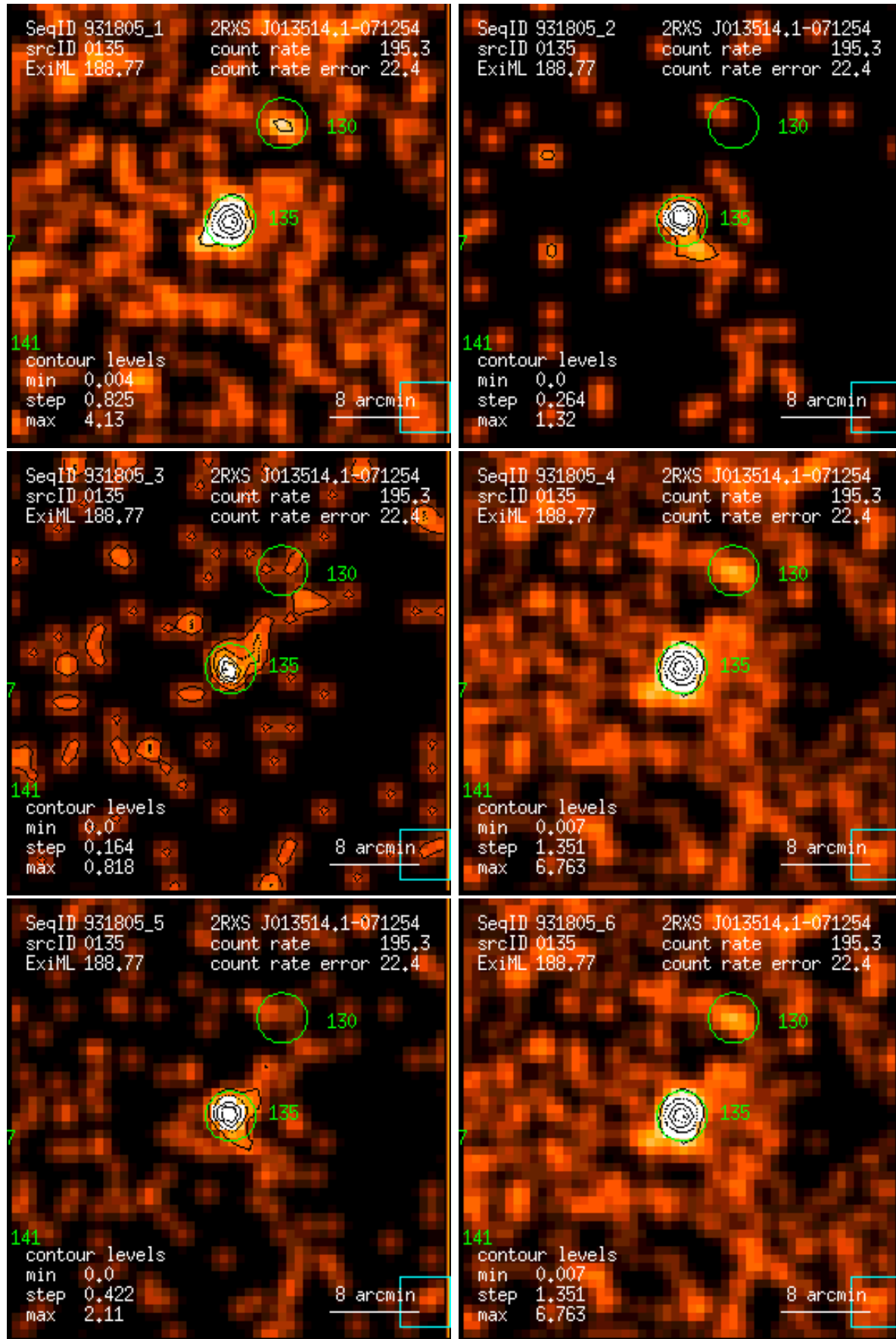
Figure 135: RASS 931805: detection 0135: band rate images, Gaussian filter: (1) PSPC channels 11 – 41, (2) 52 – 90, (3) 91 – 201, (4) 11 – 235, (5) 52 – 201, (6) 11 – 201. Broad band rates in counts/ks. Band rate contour levels in counts/ks/arcmin 2 .
