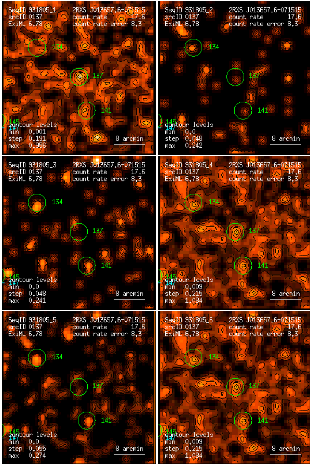
Figure 137: RASS 931805: detection 0137: band rate images, Gaussian filter: (1) PSPPC channels 11 – 41, (2) 52 – 90, (3) 91 – 201, (4) 11 – 235, (5) 52 – 201, (6) 11 – 201. Broad band rates in counts/ks. Band rate contour levels in counts/ks/arcmin 2 .
