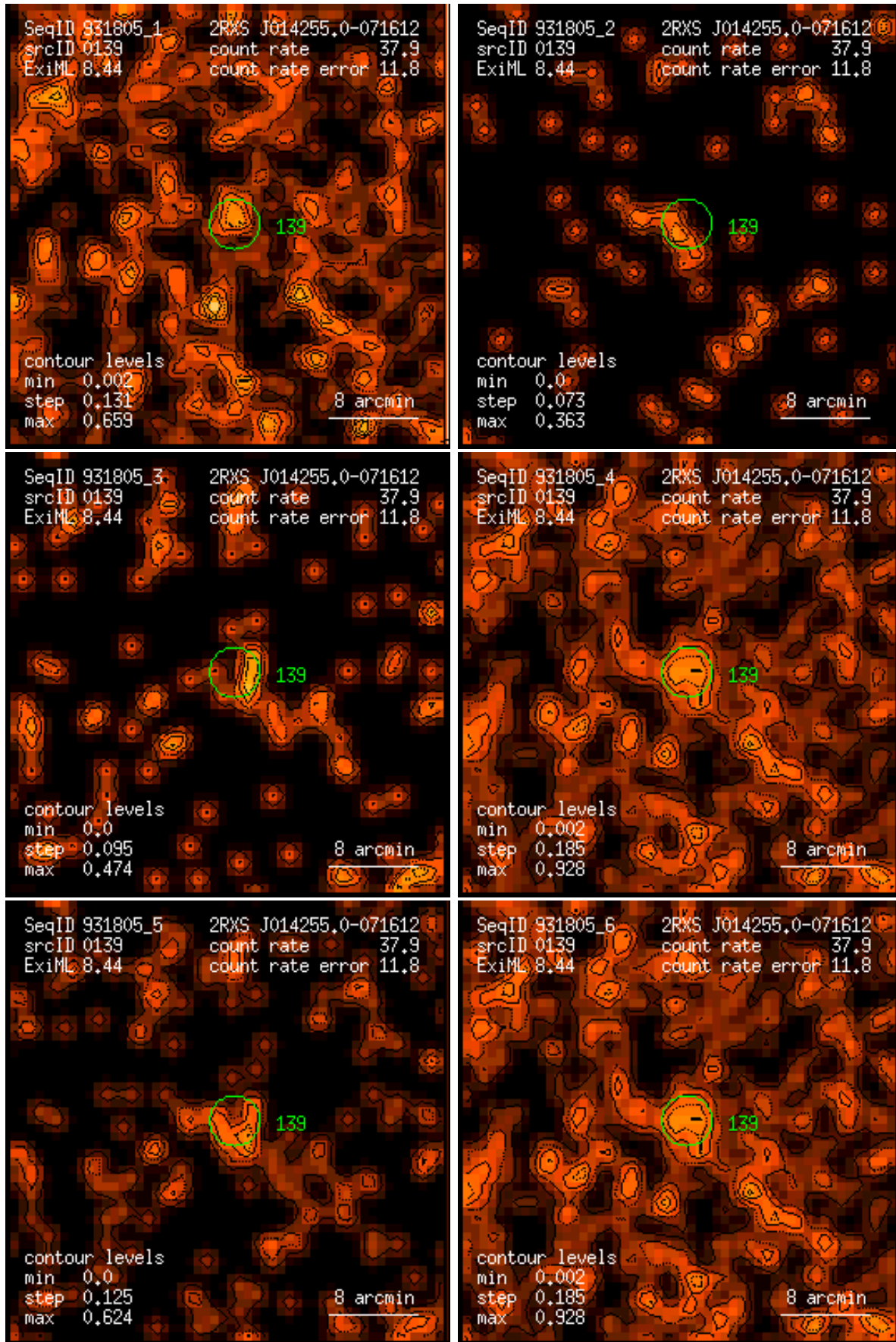
Figure 139: RASS 931805: detection 0139: band rate images, Gaussian filter: (1) PSPC channels 11 – 41, (2) 52 – 90, (3) 91 – 201, (4) 11 – 235, (5) 52 – 201, (6) 11 – 201. Broad band rates in counts/ks. Band rate contour levels in counts/ks/arcmin 2 .
