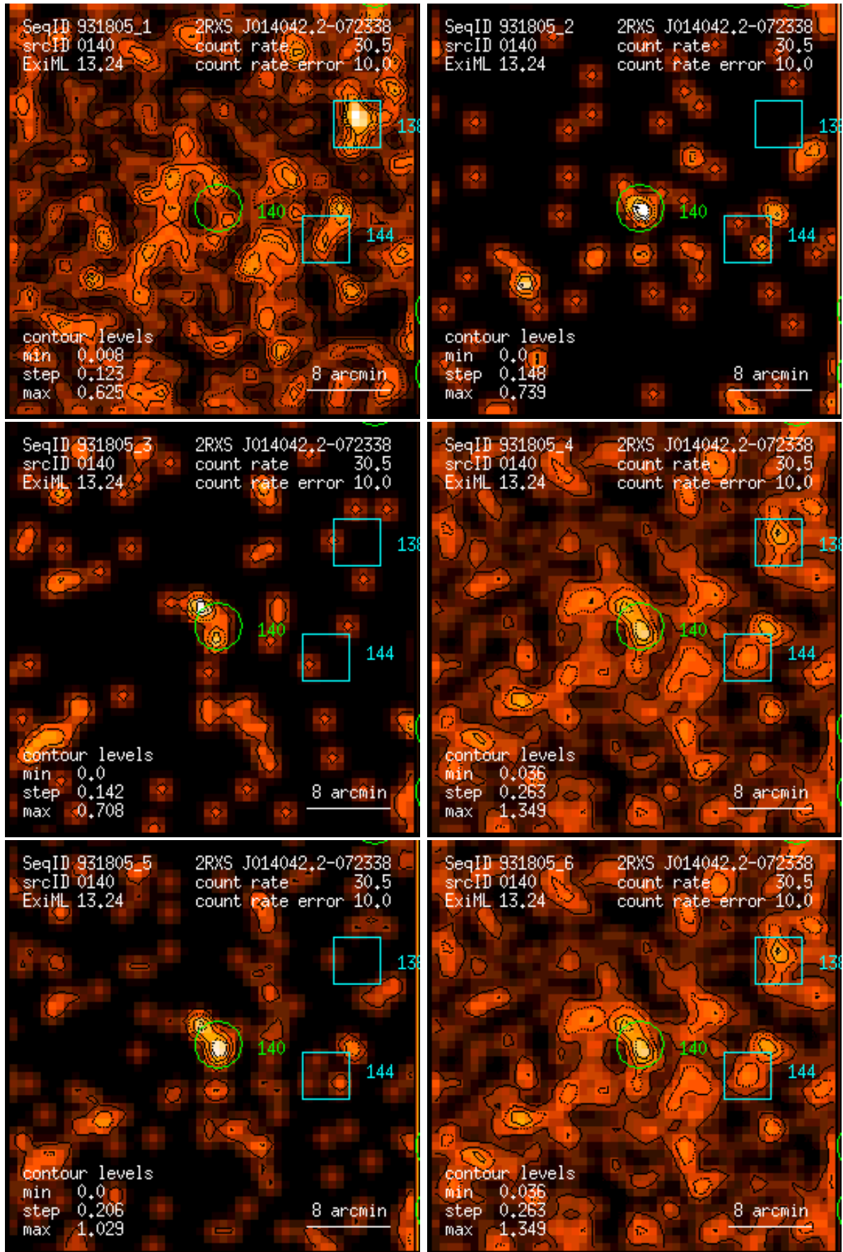
Figure 140: RASS 931805: detection 0140: band rate images, Gaussian filter: (1) PSPC channels 11 – 41, (2) 52 – 90, (3) 91 – 201, (4) 11 – 235, (5) 52 – 201, (6) 11 – 201. Broad band rates in counts/ks. Band rate contour levels in counts/ks/arcmin 2 .
