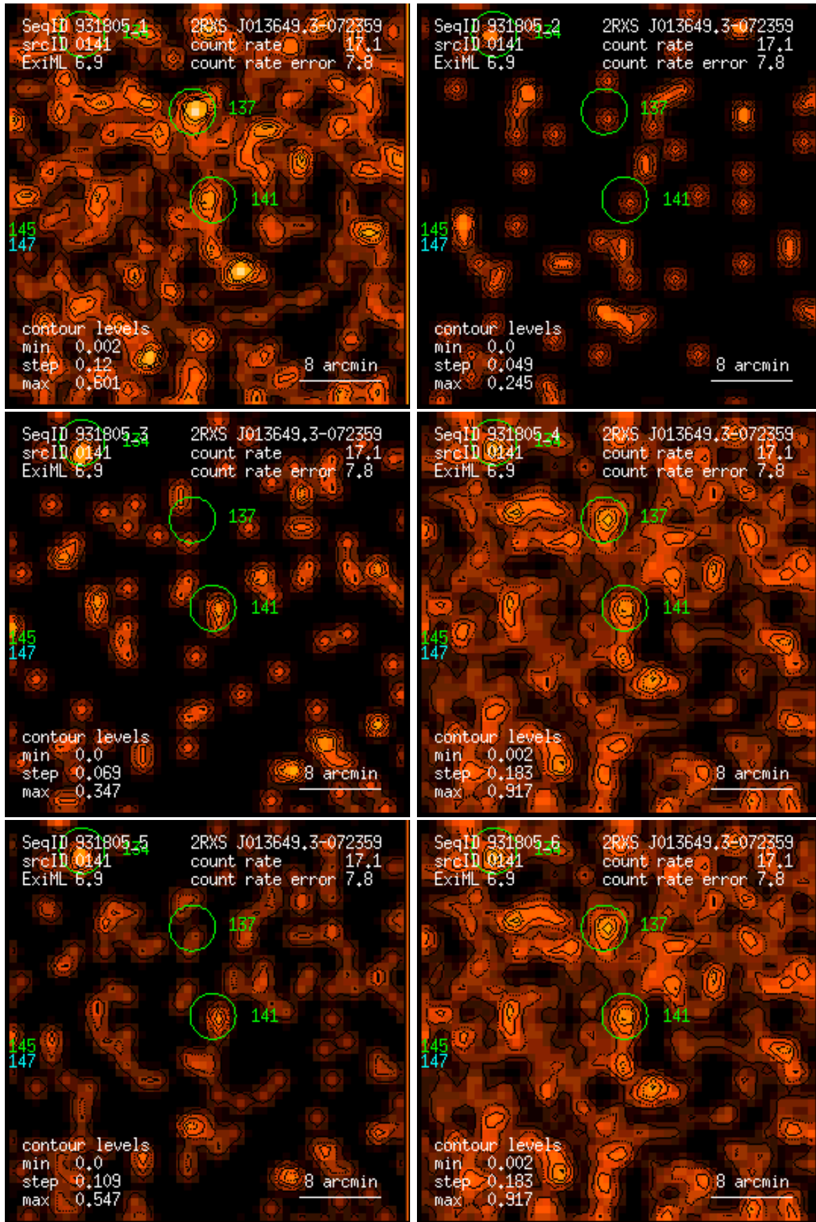
Figure 141: RASS 931805: detection 0141: band rate images, Gaussian filter: (1) PSPC channels 11 – 41, (2) 52 – 90, (3) 91 – 201, (4) 11 – 235, (5) 52 – 201, (6) 11 – 201. Broad band rates in counts/ks. Band rate contour levels in counts/ks/arcmin 2 .
