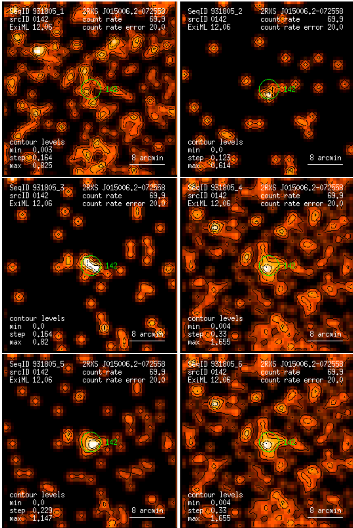
Figure 142: RASS 931805: detection 0142: band rate images, Gaussian filter: (1) PSPC channels 11 – 41, (2) 52 – 90, (3) 91 – 201, (4) 11 – 235, (5) 52 – 201, (6) 11 – 201. Broad band rates in counts/ks. Band rate contour levels in counts/ks/arcmin 2 .
