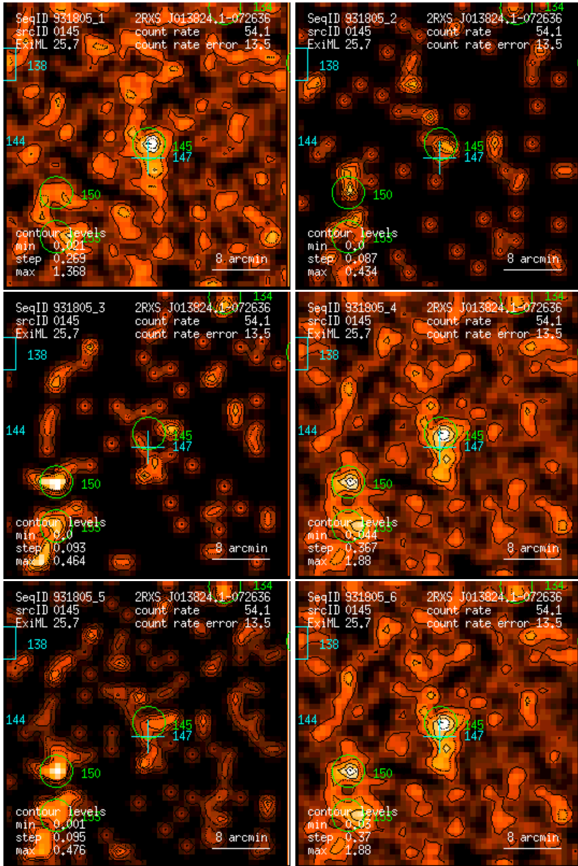
Figure 145: RASS 931805: detection 0145: band rate images, Gaussian filter: (1) PSPC channels 11 – 41, (2) 52 – 90, (3) 91 – 201, (4) 11 – 235, (5) 52 – 201, (6) 11 – 201. Broad band rates in counts/ks. Band rate contour levels in counts/ks/arcmin 2 .
