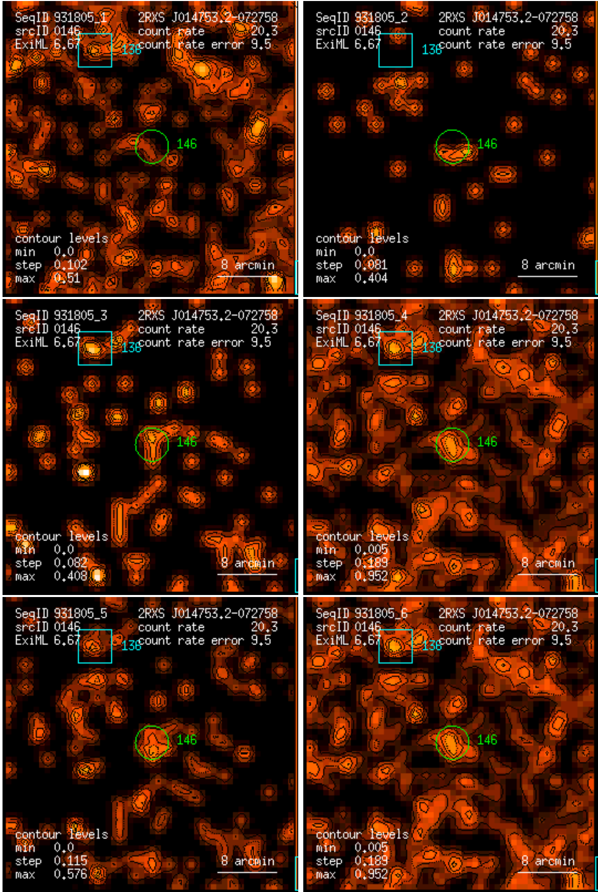
Figure 146: RASS 931805: detection 0146: band rate images, Gaussian filter: (1) PSPC channels 11 – 41, (2) 52 – 90, (3) 91 – 201, (4) 11 – 235, (5) 52 – 201, (6) 11 – 201. Broad band rates in counts/ks. Band rate contour levels in counts/ks/arcmin 2 .
