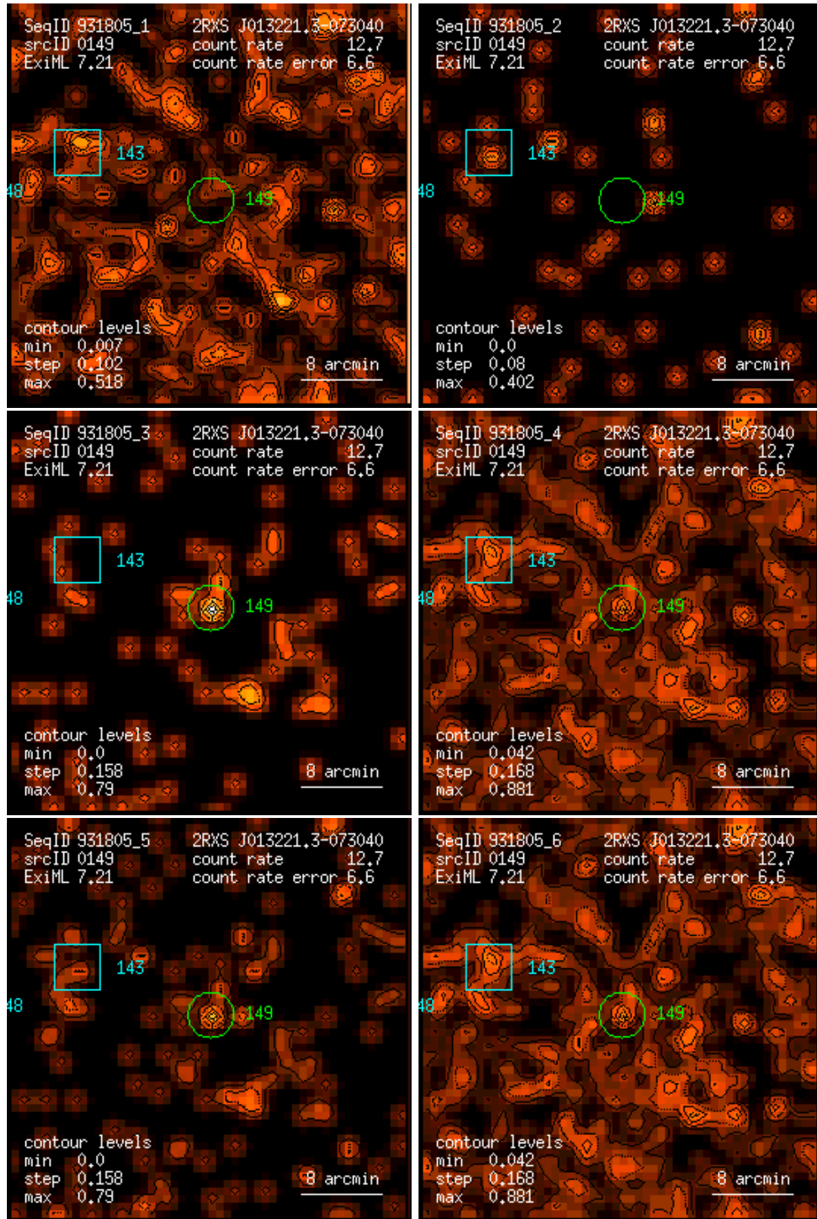
Figure 149: RASS 931805: detection 0149: band rate images, Gaussian filter: (1) PSPC channels 11 – 41, (2) 52 – 90, (3) 91 – 201, (4) 11 – 235, (5) 52 – 201, (6) 11 – 201. Broad band rates in counts/ks. Band rate contour levels in counts/ks/arcmin 2 .
