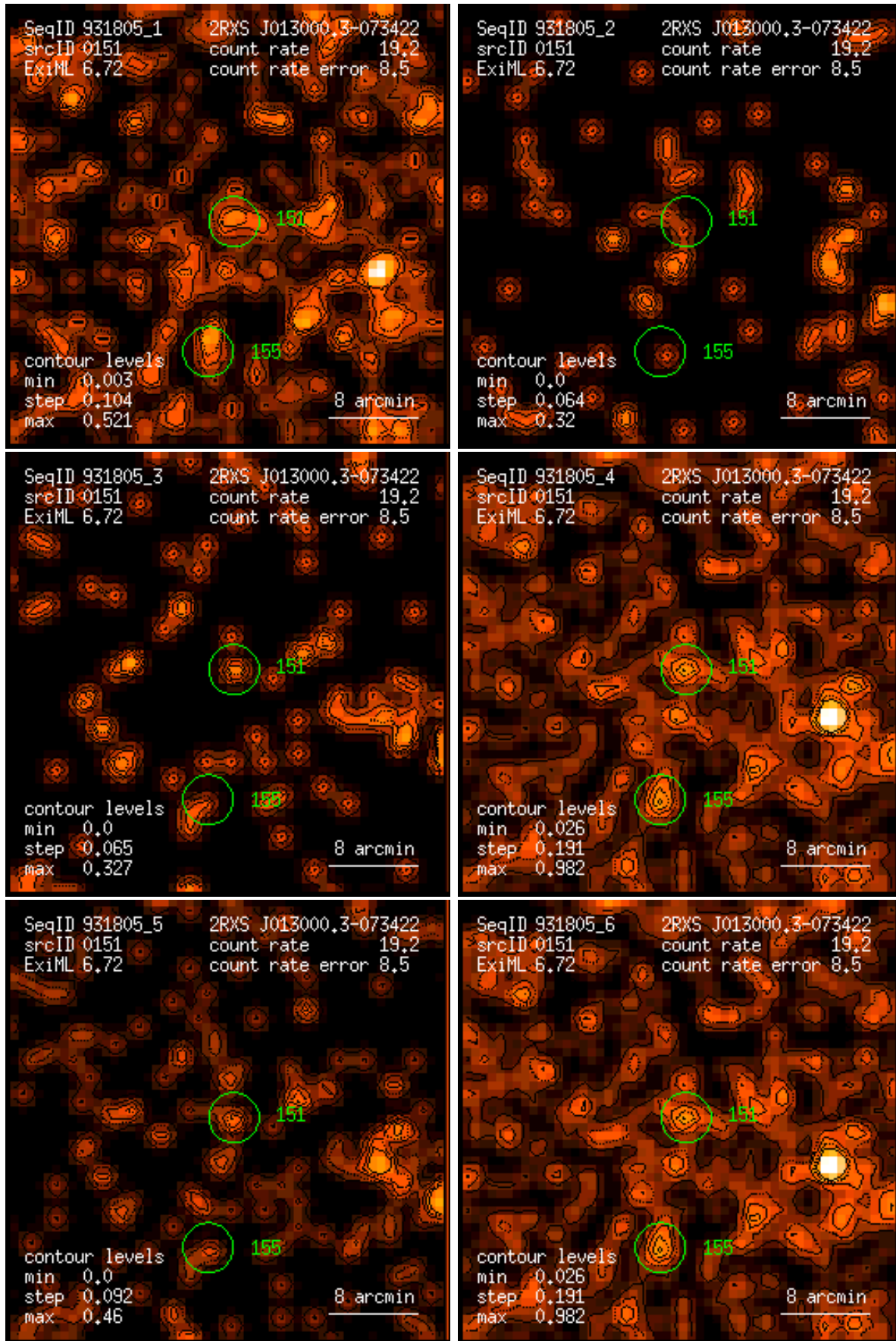
Figure 151: RASS 931805: detection 0151: band rate images, Gaussian filter: (1) PSPC channels 11 – 41, (2) 52 – 90, (3) 91 – 201, (4) 11 – 235, (5) 52 – 201, (6) 11 – 201. Broad band rates in counts/ks. Band rate contour levels in counts/ks/arcmin 2 .
