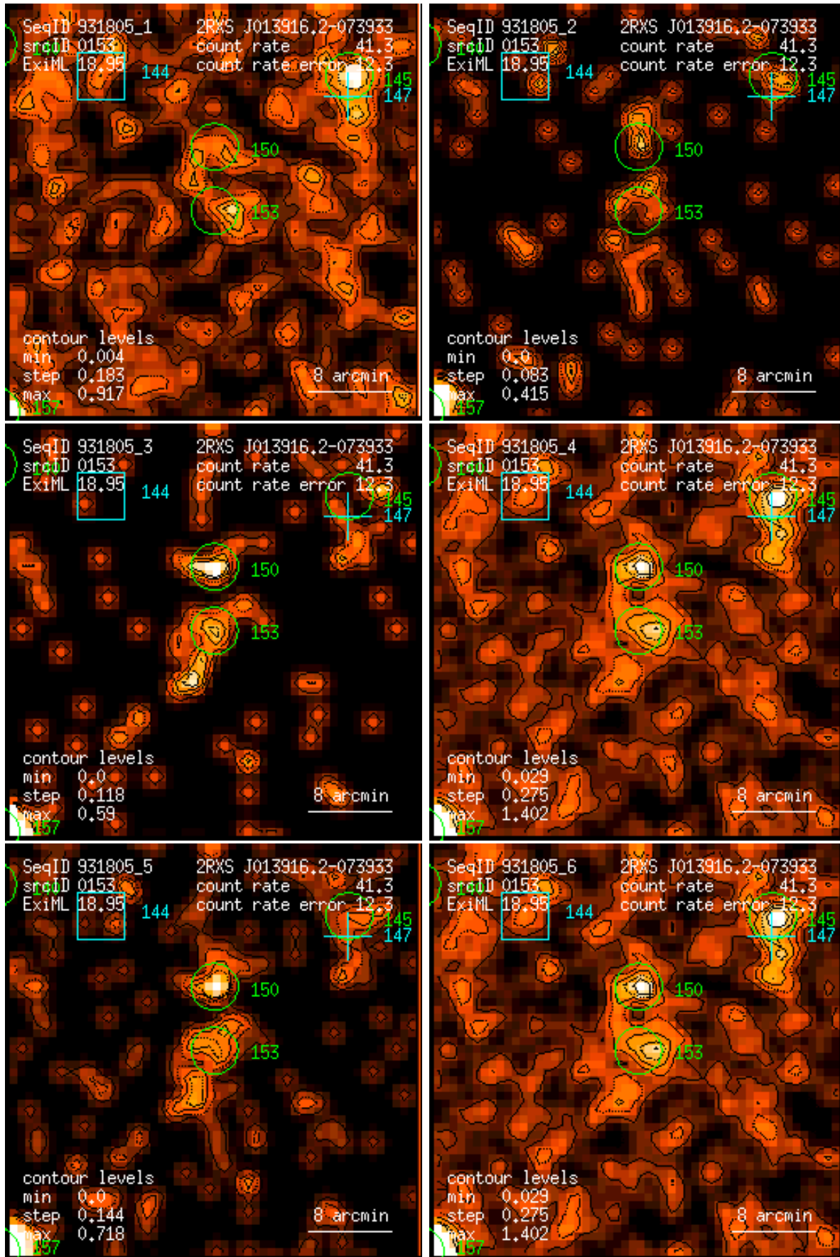
Figure 153: RASS 931805: detection 0153: band rate images, Gaussian filter: (1) PSPC channels 11 – 41, (2) 52 – 90, (3) 91 – 201, (4) 11 – 235, (5) 52 – 201, (6) 11 – 201. Broad band rates in counts/ks. Band rate contour levels in counts/ks/arcmin 2 .
