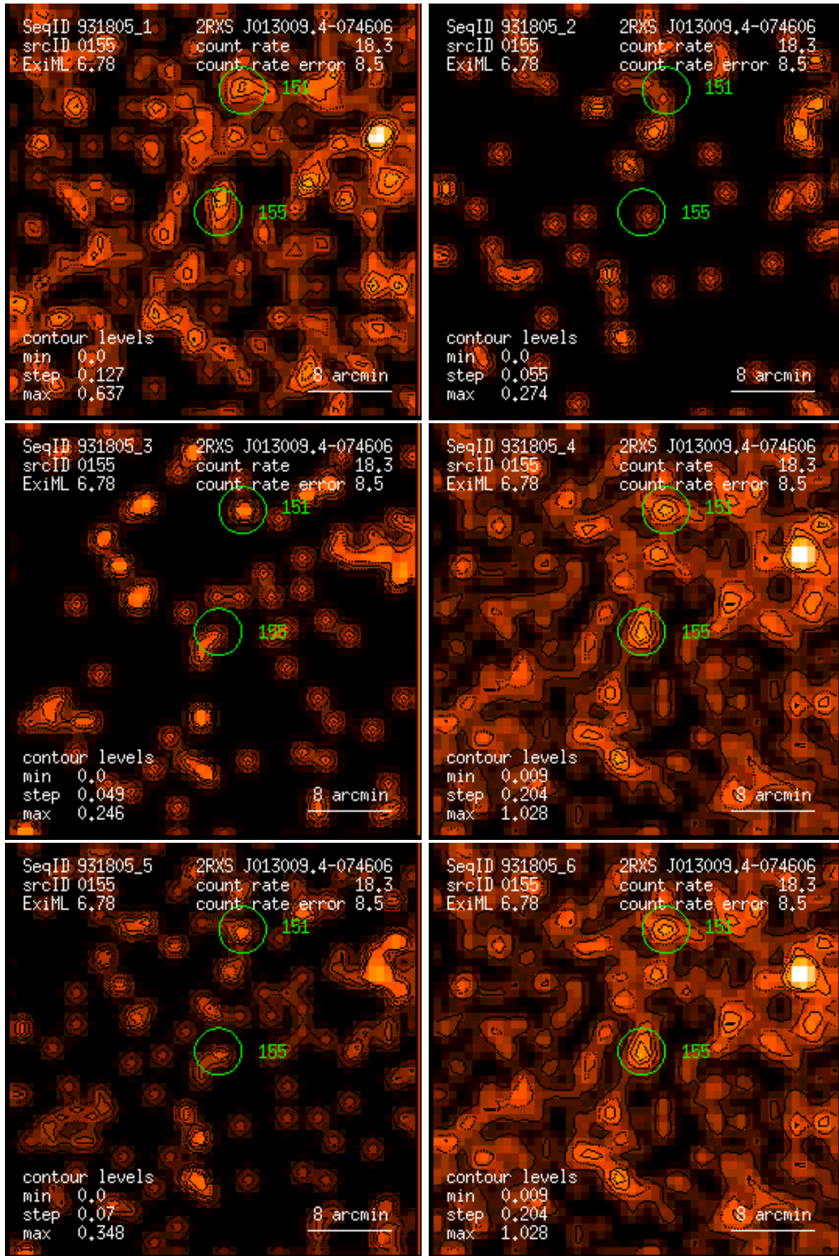
Figure 155: RASS 931805: detection 0155: band rate images, Gaussian filter: (1) PSPC channels 11 – 41, (2) 52 – 90, (3) 91 – 201, (4) 11 – 235, (5) 52 – 201, (6) 11 – 201. Broad band rates in counts/ks. Band rate contour levels in counts/ks/arcmin 2 .
