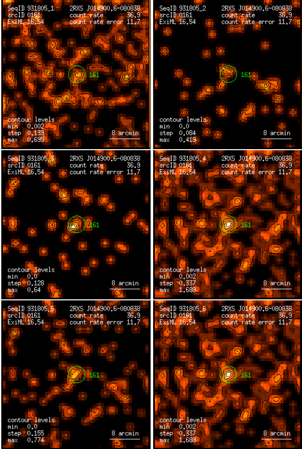
Figure 161: RASS 931805: detection 0161: band rate images, Gaussian filter: (1) PSPC channels 11 – 41, (2) 52 – 90, (3) 91 – 201, (4) 11 – 235, (5) 52 – 201, (6) 11 – 201. Broad band rates in counts/ks. Band rate contour levels in counts/ks/arcmin 2 .
