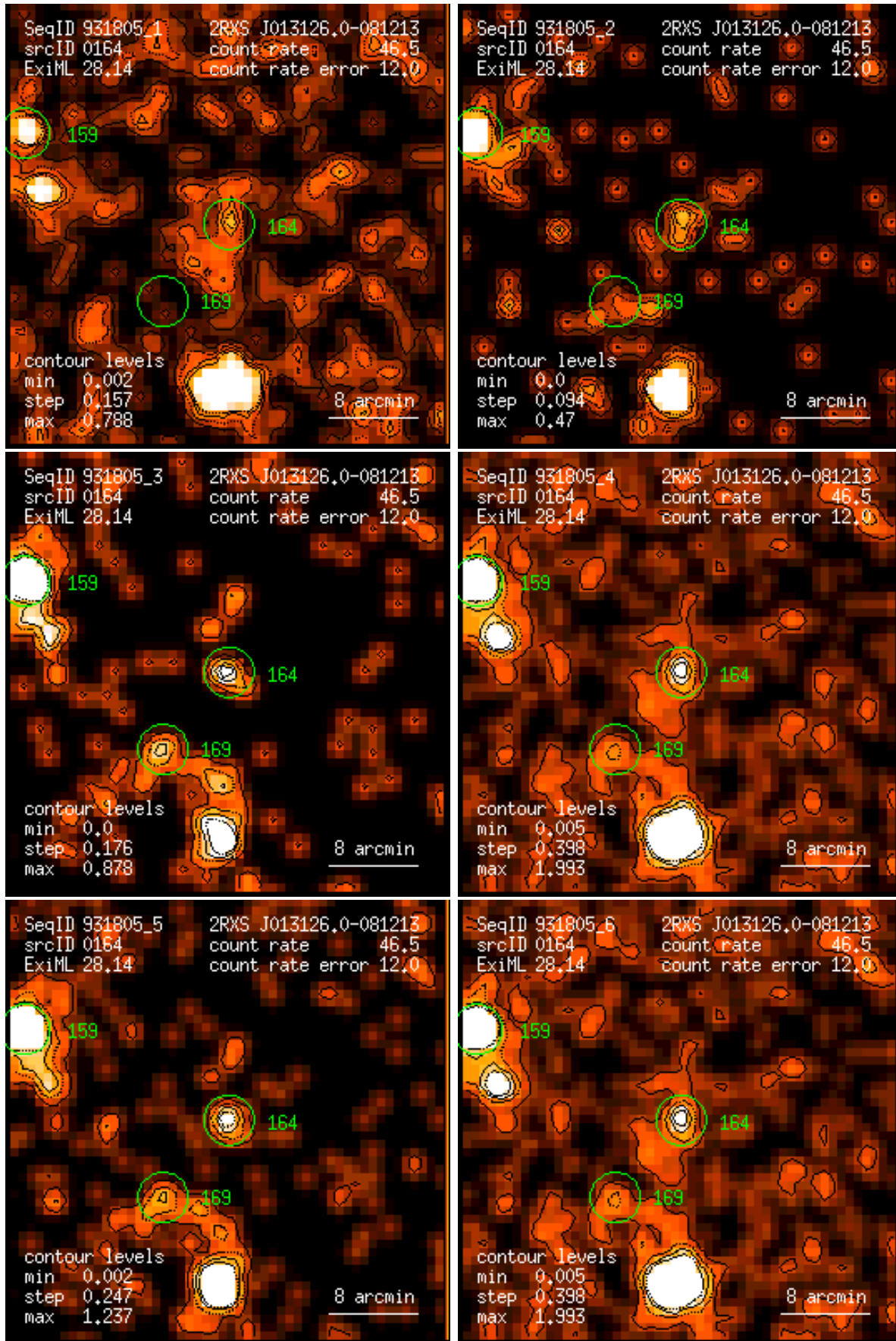
Figure 164: RASS 931805: detection 0164: band rate images, Gaussian filter: (1) PSPC channels 11 – 41, (2) 52 – 90, (3) 91 – 201, (4) 11 – 235, (5) 52 – 201, (6) 11 – 201. Broad band rates in counts/ks. Band rate contour levels in counts/ks/arcmin 2 .
