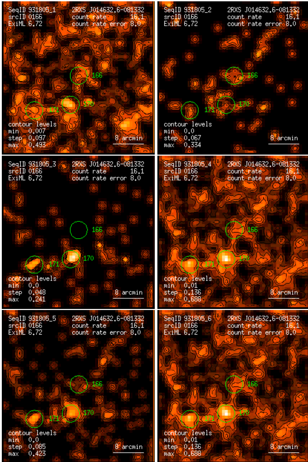
Figure 166: RASS 931805: detection 0166: band rate images, Gaussian filter: (1) PSPPC channels 11 – 41, (2) 52 – 90, (3) 91 – 201, (4) 11 – 235, (5) 52 – 201, (6) 11 – 201. Broad band rates in counts/ks. Band rate contour levels in counts/ks/arcmin 2 .
