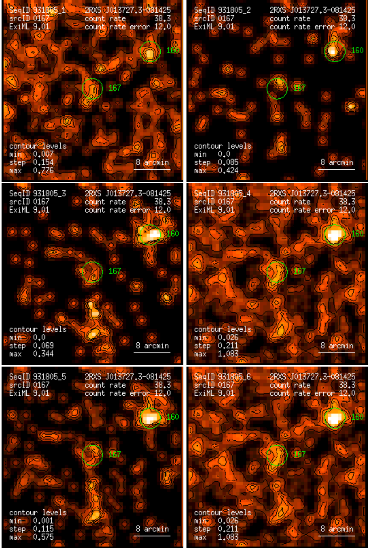
Figure 167: RASS 931805: detection 0167: band rate images, Gaussian filter: (1) PSPC channels 11 – 41, (2) 52 – 90, (3) 91 – 201, (4) 11 – 235, (5) 52 – 201, (6) 11 – 201. Broad band rates in counts/ks. Band rate contour levels in counts/ks/arcmin 2 .
