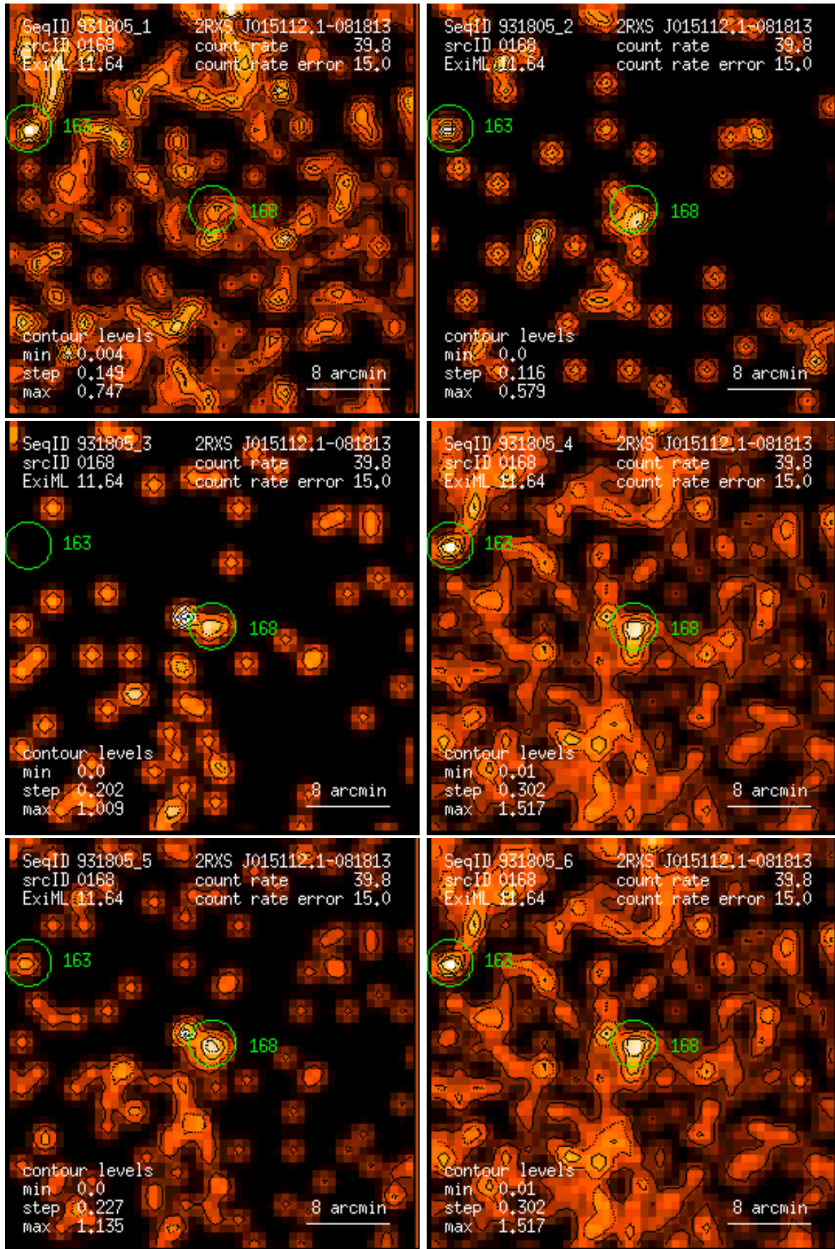
Figure 168: RASS 931805: detection 0168: band rate images, Gaussian filter: (1) PSPC channels 11 – 41, (2) 52 – 90, (3) 91 – 201, (4) 11 – 235, (5) 52 – 201, (6) 11 – 201. Broad band rates in counts/ks. Band rate contour levels in counts/ks/arcmin 2 .
