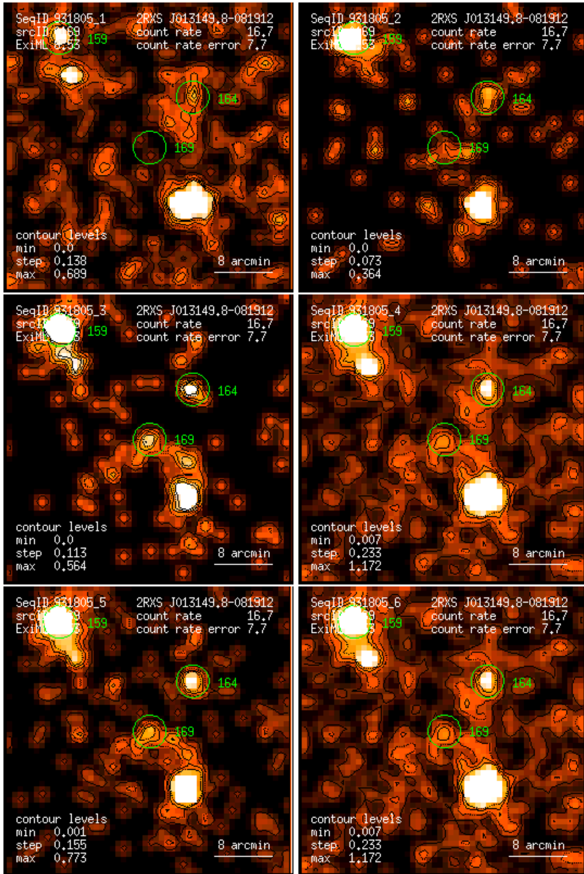
Figure 169: RASS 931805: detection 0169: band rate images, Gaussian filter: (1) PSPC channels 11 – 41, (2) 52 – 90, (3) 91 – 201, (4) 11 – 235, (5) 52 – 201, (6) 11 – 201. Broad band rates in counts/ks. Band rate contour levels in counts/ks/arcmin 2 .
