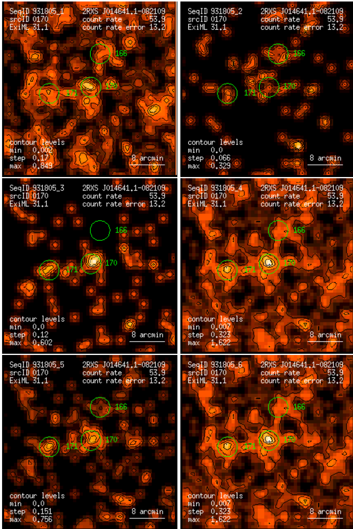
Figure 170: RASS 931805: detection 0170: band rate images, Gaussian filter: (1) PSPC channels 11 – 41, (2) 52 – 90, (3) 91 – 201, (4) 11 – 235, (5) 52 – 201, (6) 11 – 201. Broad band rates in counts/ks. Band rate contour levels in counts/ks/arcmin 2 .
