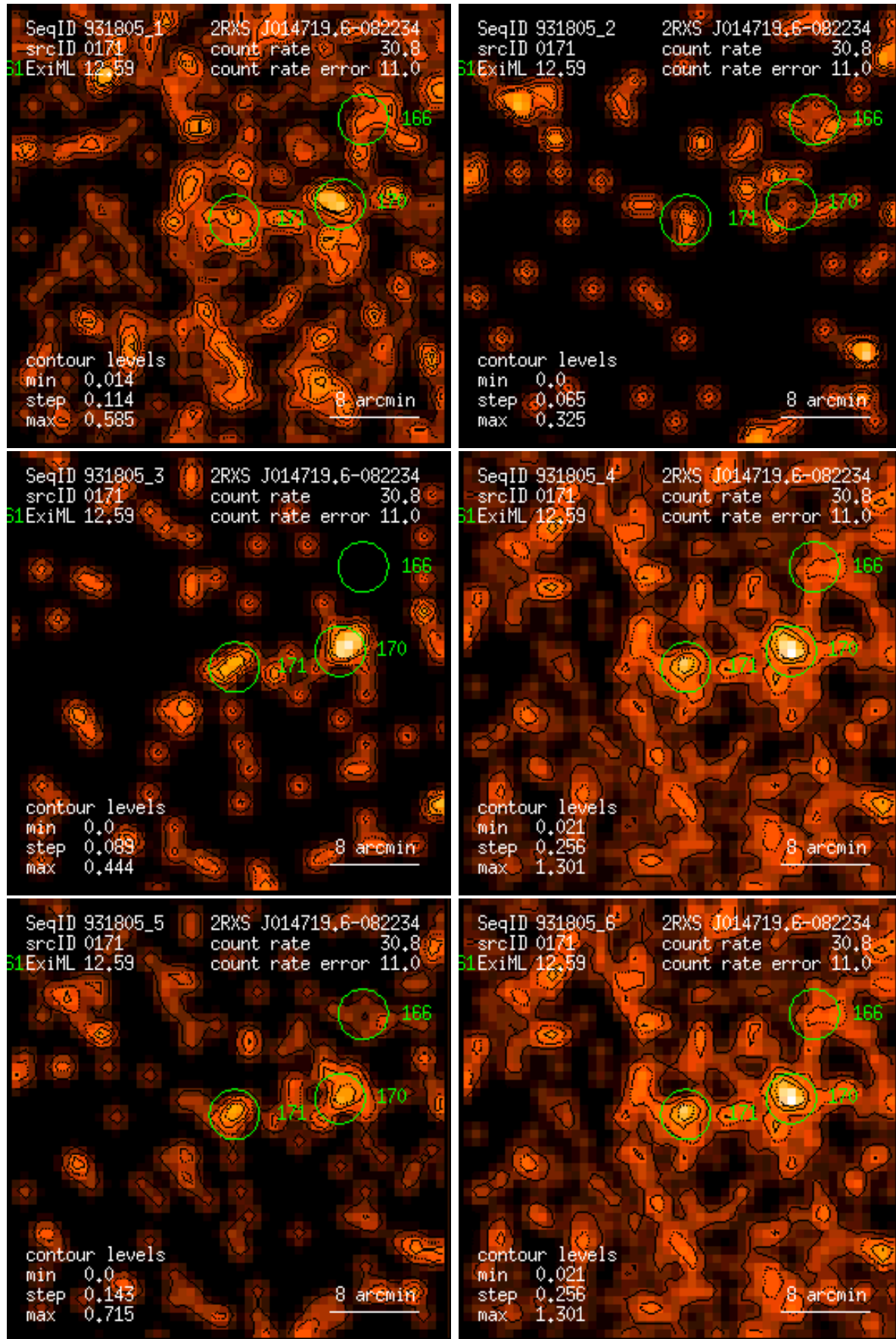
Figure 171: RASS 931805: detection 0171: band rate images, Gaussian filter: (1) PSPC channels 11 – 41, (2) 52 – 90, (3) 91 – 201, (4) 11 – 235, (5) 52 – 201, (6) 11 – 201. Broad band rates in counts/ks. Band rate contour levels in counts/ks/arcmin 2 .
