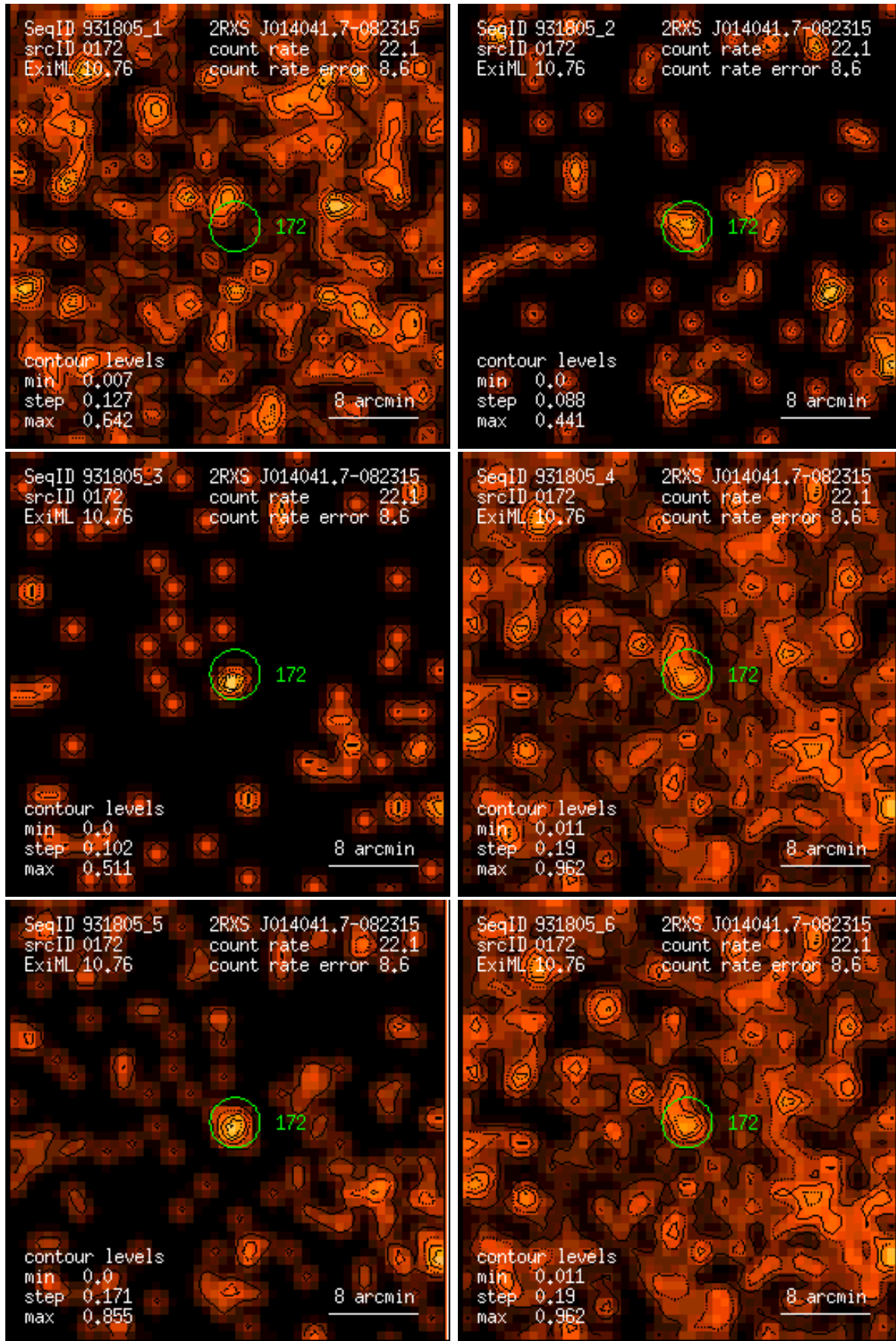
Figure 172: RASS 931805: detection 0172: band rate images, Gaussian filter: (1) PSPC channels 11 – 41, (2) 52 – 90, (3) 91 – 201, (4) 11 – 235, (5) 52 – 201, (6) 11 – 201. Broad band rates in counts/ks. Band rate contour levels in counts/ks/arcmin 2 .
