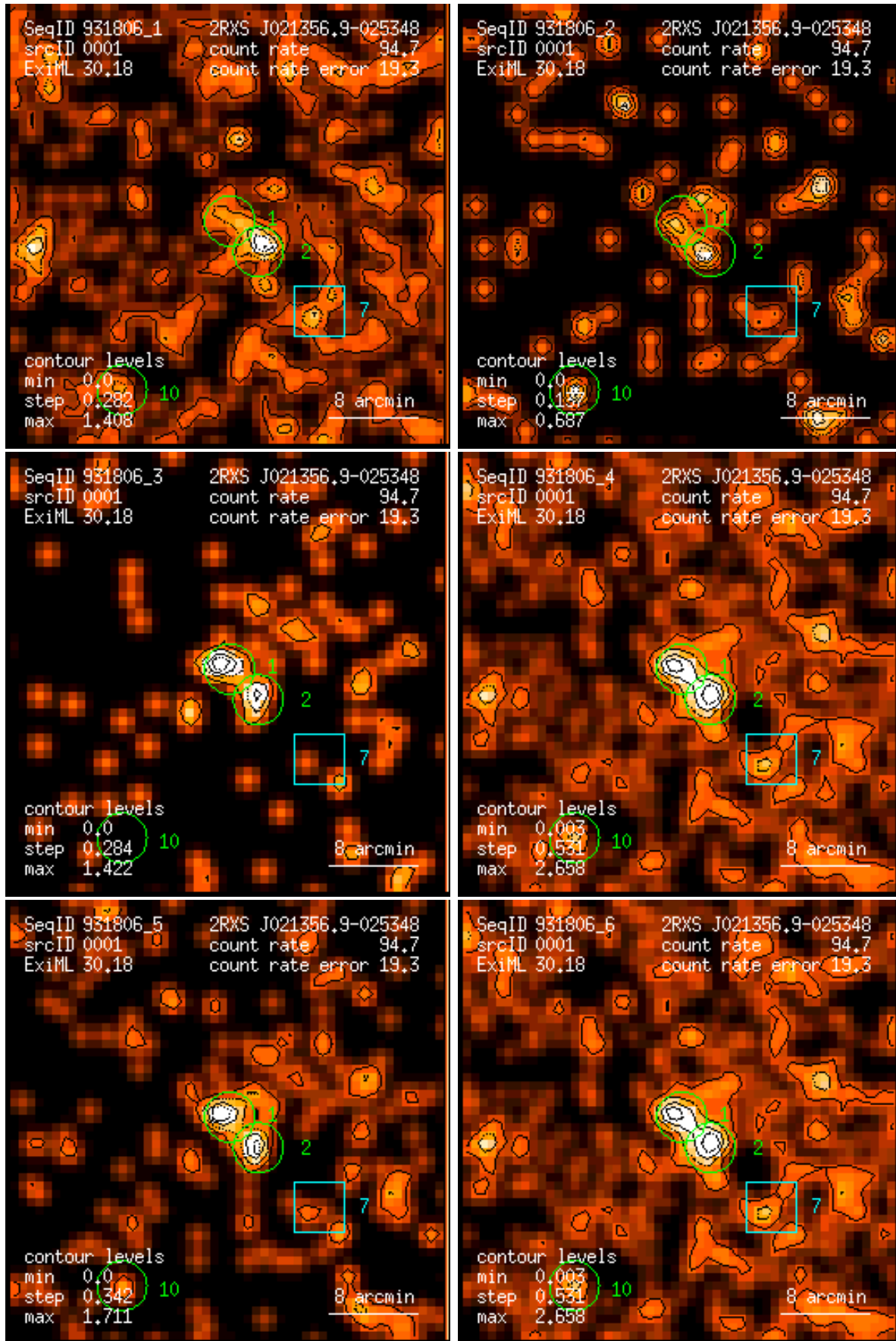
Figure 1: RASS 931806: detection 0001: band rate images, Gaussian filter: (1) PSPC channels 11 – 41, (2) 52 – 90, (3) 91 – 201, (4) 11 – 235, (5) 52 – 201, (6) 11 – 201. Broad band rates in counts/ks. Band rate contour levels in counts/ks/arcmin 2 .
