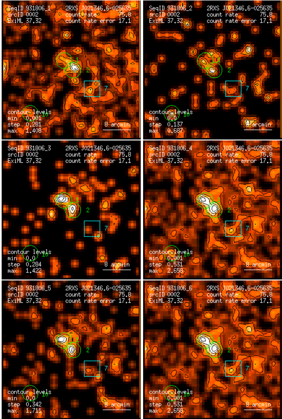
Figure 2: RASS 931806: detection 0002: band rate images, Gaussian filter: (1) PSPC channels 11 – 41, (2) 52 – 90, (3) 91 – 201, (4) 11 – 235, (5) 52 – 201, (6) 11 – 201. Broad band rates in counts/ks. Band rate contour levels in counts/ks/arcmin 2 .
