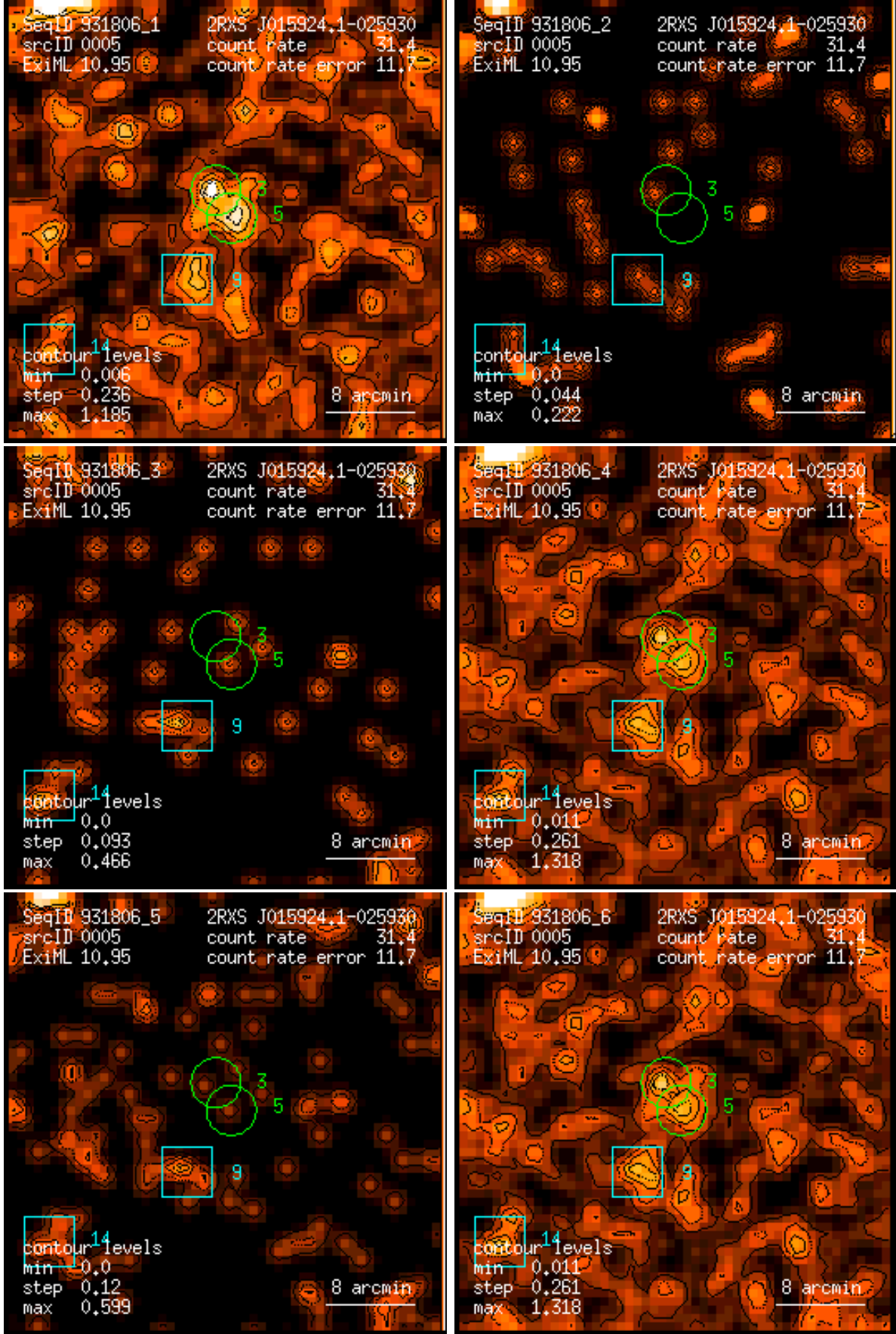
Figure 5: RASS 931806: detection 0005: band rate images, Gaussian filter: (1) PSPC channels 11 – 41, (2) 52 – 90, (3) 91 – 201, (4) 11 – 235, (5) 52 – 201, (6) 11 – 201. Broad band rates in counts/ks. Band rate contour levels in counts/ks/arcmin 2 .
