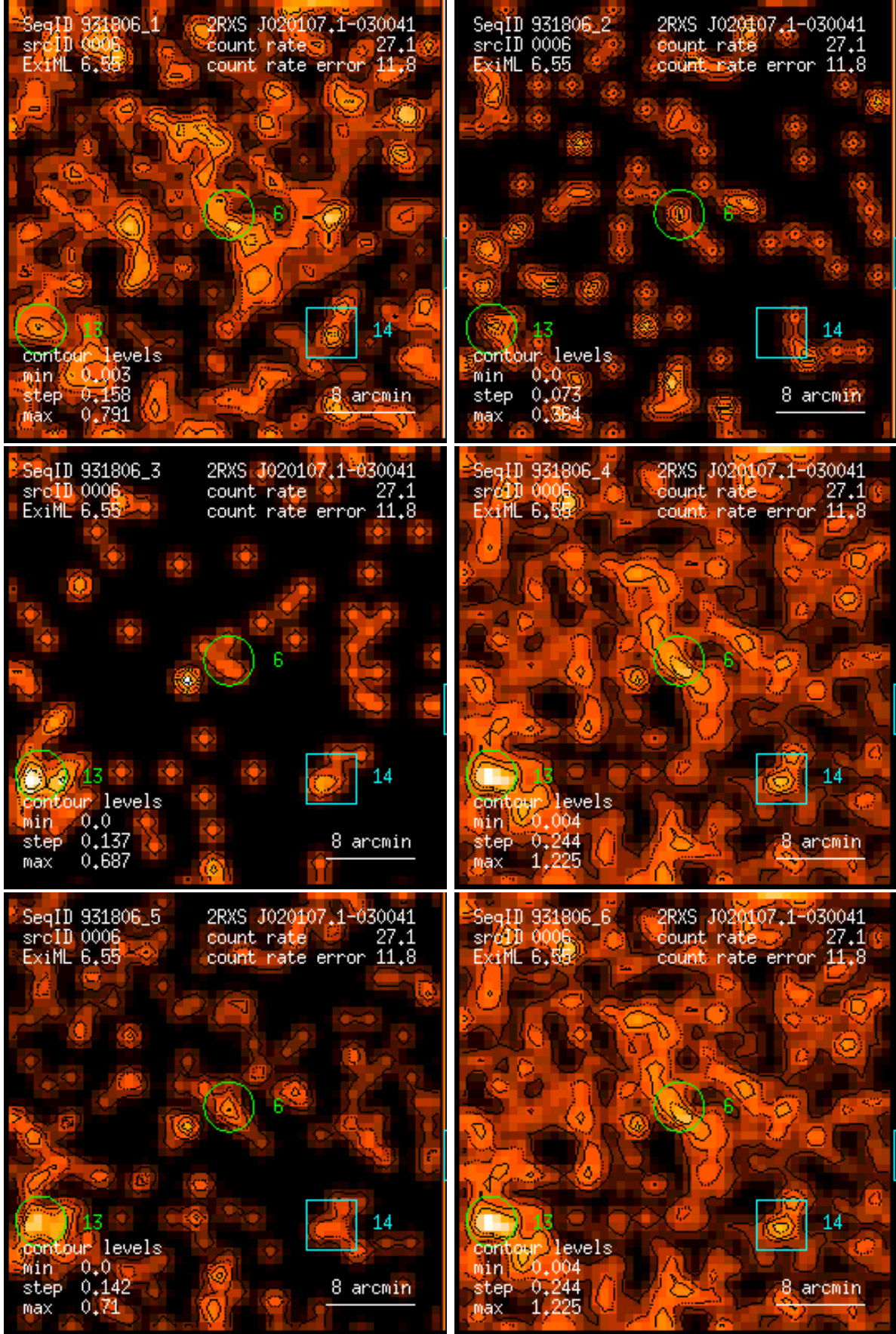
Figure 6: RASS 931806: detection 0006: band rate images, Gaussian filter: (1) PSPC channels 11 – 41, (2) 52 – 90, (3) 91 – 201, (4) 11 – 235, (5) 52 – 201, (6) 11 – 201. Broad band rates in counts/ks. Band rate contour levels in counts/ks/arcmin 2 .
