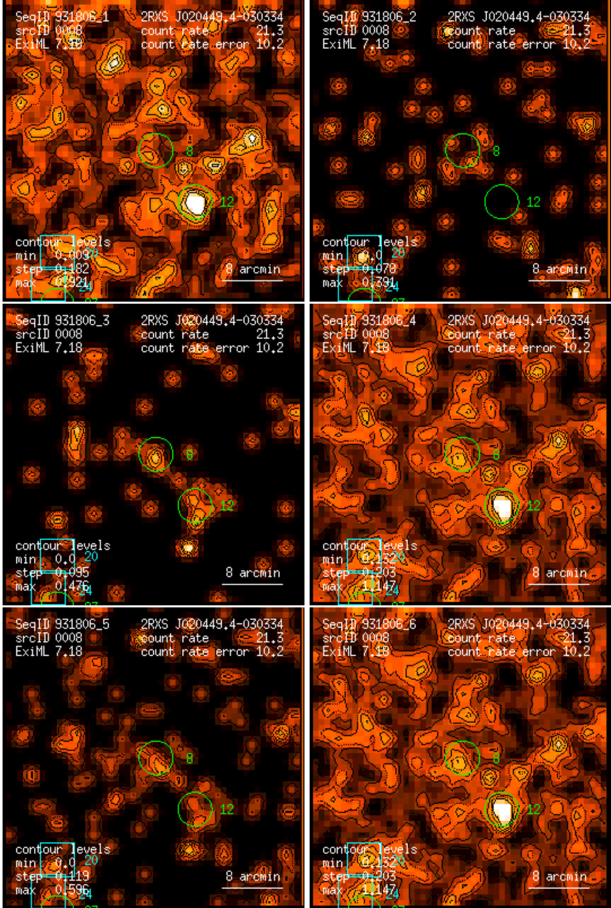
Figure 8: RASS 931806: detection 0008: band rate images, Gaussian filter: (1) PSPC channels 11 – 41, (2) 52 – 90, (3) 91 – 201, (4) 11 – 235, (5) 52 – 201, (6) 11 – 201. Broad band rates in counts/ks. Band rate contour levels in counts/ks/arcmin 2 .
