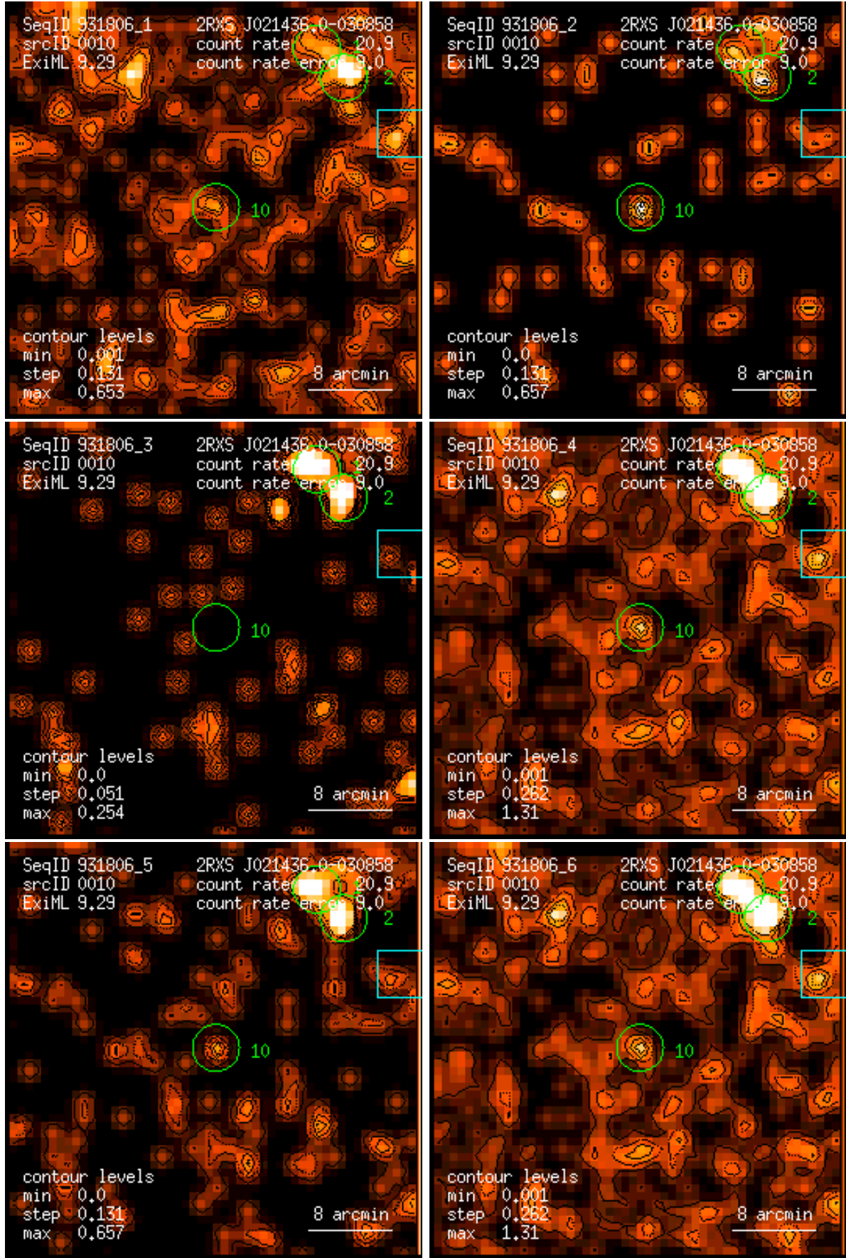
Figure 10: RASS 931806: detection 0010: band rate images, Gaussian filter: (1) PSPC channels 11 – 41, (2) 52 – 90, (3) 91 – 201, (4) 11 – 235, (5) 52 – 201, (6) 11 – 201. Broad band rates in counts/ks. Band rate contour levels in counts/ks/arcmin 2 .
