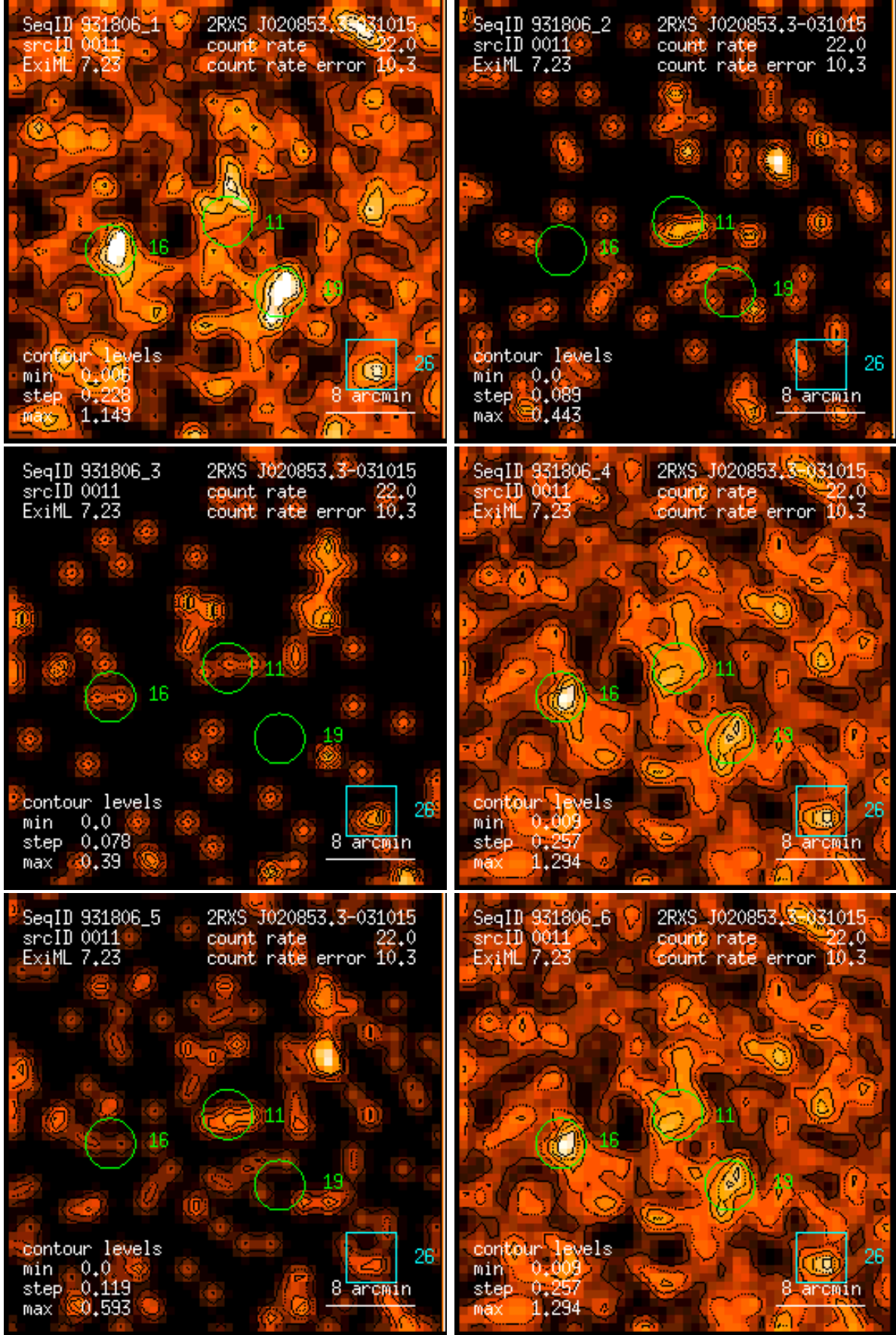
Figure 11: RASS 931806: detection 0011: band rate images, Gaussian filter: (1) PSPC channels 11 – 41, (2) 52 – 90, (3) 91 – 201, (4) 11 – 235, (5) 52 – 201, (6) 11 – 201. Broad band rates in counts/ks. Band rate contour levels in counts/ks/arcmin 2 .
