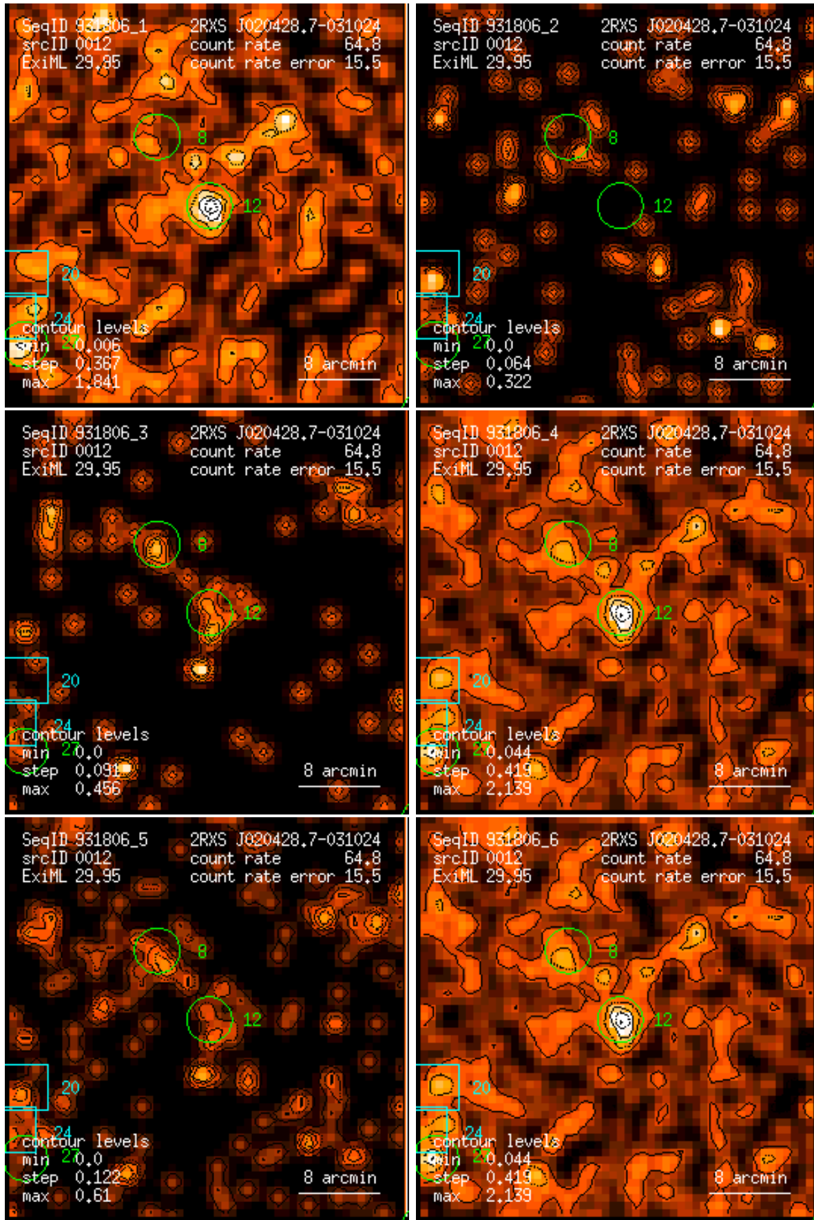
Figure 12: RASS 931806: detection 0012: band rate images, Gaussian filter: (1) PSPC channels 11 – 41, (2) 52 – 90, (3) 91 – 201, (4) 11 – 235, (5) 52 – 201, (6) 11 – 201. Broad band rates in counts/ks. Band rate contour levels in counts/ks/arcmin 2 .
