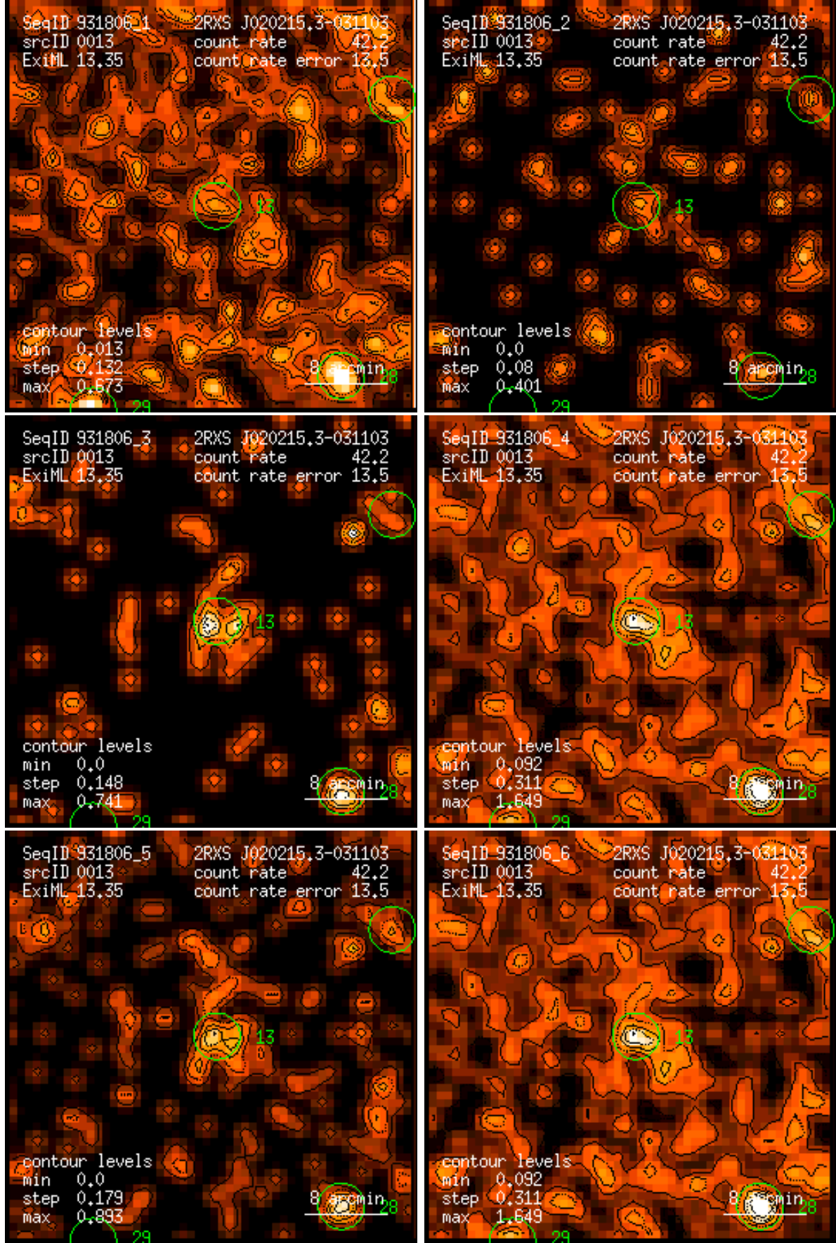
Figure 13: RASS 931806: detection 0013: band rate images, Gaussian filter: (1) PSPC channels 11 – 41, (2) 52 – 90, (3) 91 – 201, (4) 11 – 235, (5) 52 – 201, (6) 11 – 201. Broad band rates in counts/ks. Band rate contour levels in counts/ks/arcmin 2 .
