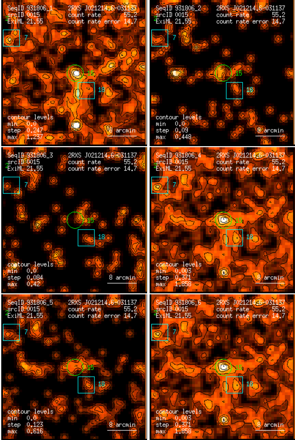
Figure 15: RASS 931806: detection 0015: band rate images, Gaussian filter: (1) PSPC channels 11 – 41, (2) 52 – 90, (3) 91 – 201, (4) 11 – 235, (5) 52 – 201, (6) 11 – 201. Broad band rates in counts/ks. Band rate contour levels in counts/ks/arcmin 2 .
