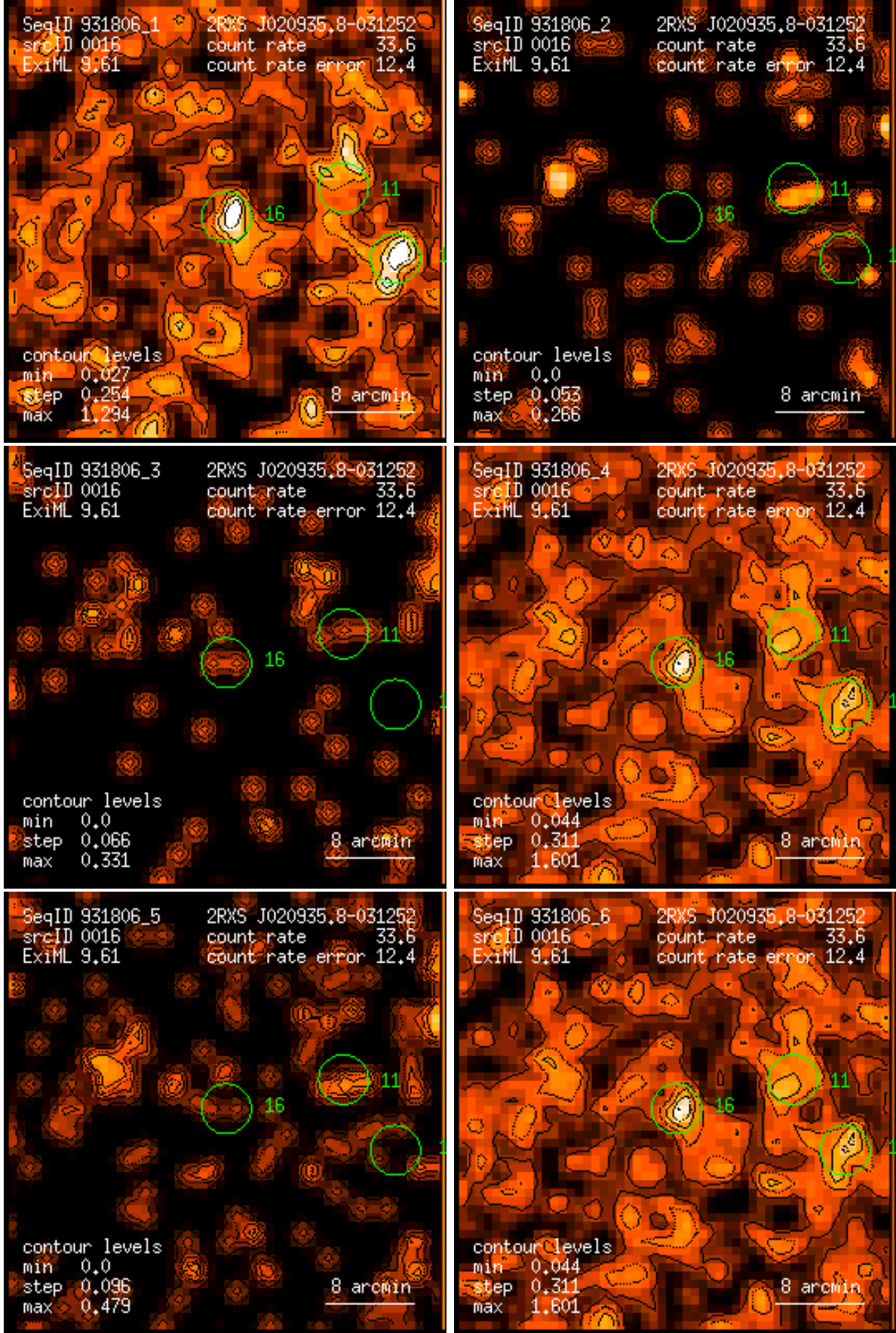
Figure 16: RASS 931806: detection 0016: band rate images, Gaussian filter: (1) PSPC channels 11 – 41, (2) 52 – 90, (3) 91 – 201, (4) 11 – 235, (5) 52 – 201, (6) 11 – 201. Broad band rates in counts/ks. Band rate contour levels in counts/ks/arcmin 2 .
