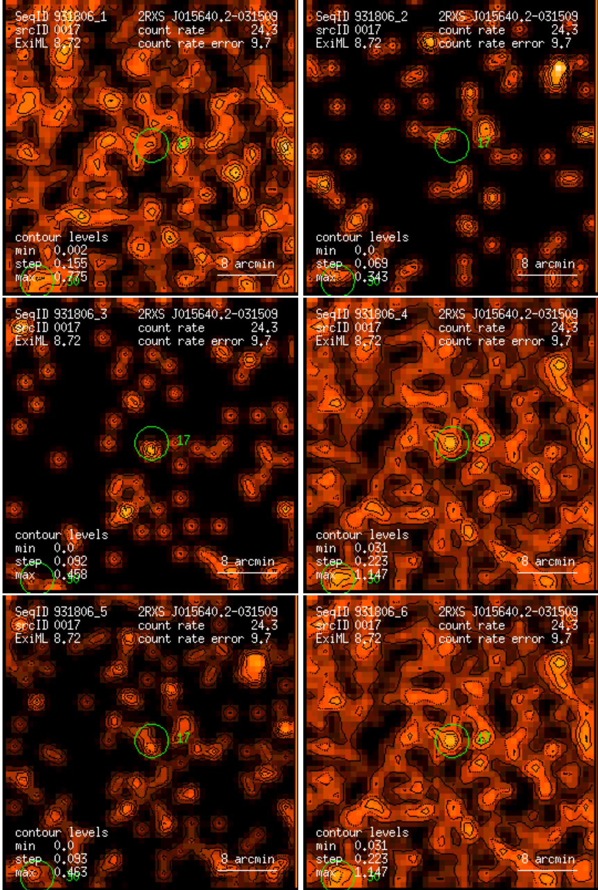
Figure 17: RASS 931806: detection 0017: band rate images, Gaussian filter: (1) PSPC channels 11 – 41, (2) 52 – 90, (3) 91 – 201, (4) 11 – 235, (5) 52 – 201, (6) 11 – 201. Broad band rates in counts/ks. Band rate contour levels in counts/ks/arcmin 2 .
