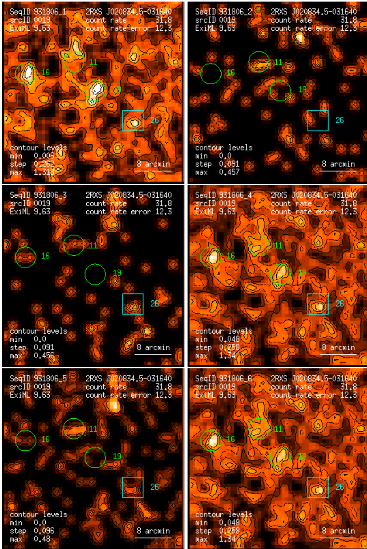
Figure 19: RASS 931806: detection 0019: band rate images, Gaussian filter: (1) PSPC channels 11 – 41, (2) 52 – 90, (3) 91 – 201, (4) 11 – 235, (5) 52 – 201, (6) 11 – 201. Broad band rates in counts/ks. Band rate contour levels in counts/ks/arcmin 2 .
