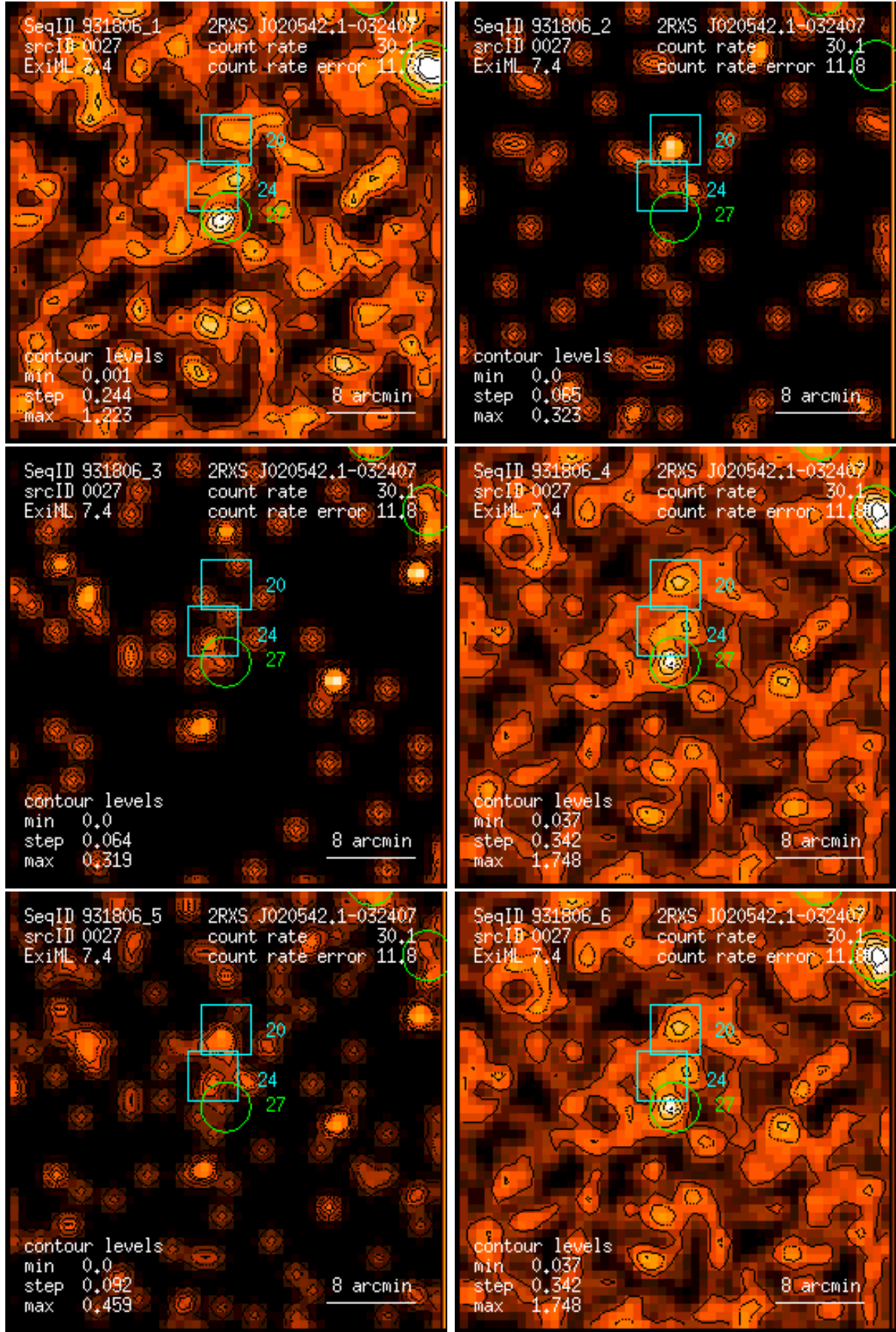
Figure 27: RASS 931806: detection 0027: band rate images, Gaussian filter: (1) PSPC channels 11 – 41, (2) 52 – 90, (3) 91 – 201, (4) 11 – 235, (5) 52 – 201, (6) 11 – 201. Broad band rates in counts/ks. Band rate contour levels in counts/ks/arcmin 2 .
